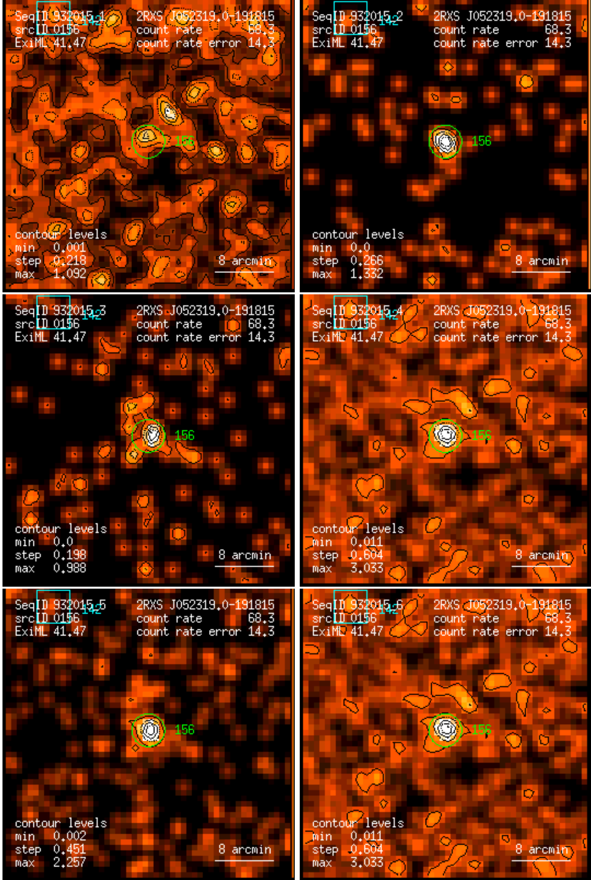
Figure 156: RASS 932015: detection 0156: band rate images, Gaussian filter: (1) PSPC channels 11 – 41, (2) 52 – 90, (3) 91 – 201, (4) 11 – 235, (5) 52 – 201, (6) 11 – 201. Broad band rates in counts/ks. Band rate contour levels in counts/ks/arcmin 2 .
