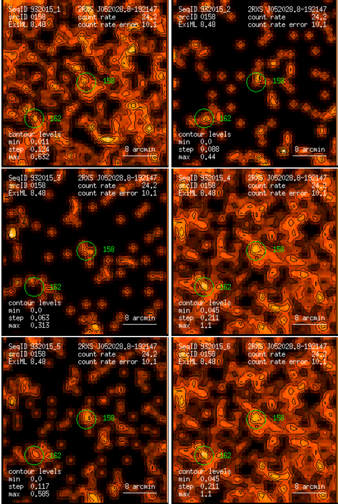
Figure 158: RASS 932015: detection 0158: band rate images, Gaussian filter: (1) PSPC channels 11 – 41, (2) 52 – 90, (3) 91 – 201, (4) 11 – 235, (5) 52 – 201, (6) 11 – 201. Broad band rates in counts/ks. Band rate contour levels in counts/ks/arcmin 2 .
