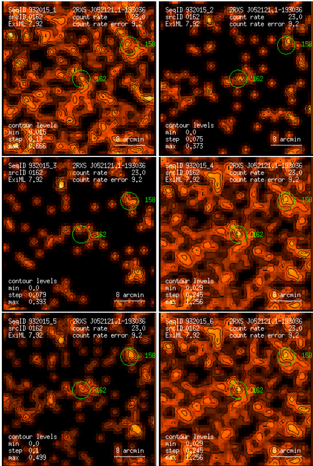
Figure 162: RASS 932015: detection 0162: band rate images, Gaussian filter: (1) PSPC channels 11 – 41, (2) 52 – 90, (3) 91 – 201, (4) 11 – 235, (5) 52 – 201, (6) 11 – 201. Broad band rates in counts/ks. Band rate contour levels in counts/ks/arcmin 2 .
