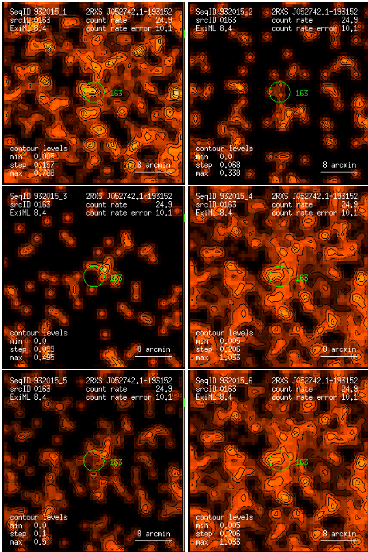
Figure 163: RASS 932015: detection 0163: band rate images, Gaussian filter: (1) PSPC channels 11 – 41, (2) 52 – 90, (3) 91 – 201, (4) 11 – 235, (5) 52 – 201, (6) 11 – 201. Broad band rates in counts/ks. Band rate contour levels in counts/ks/arcmin 2 .
