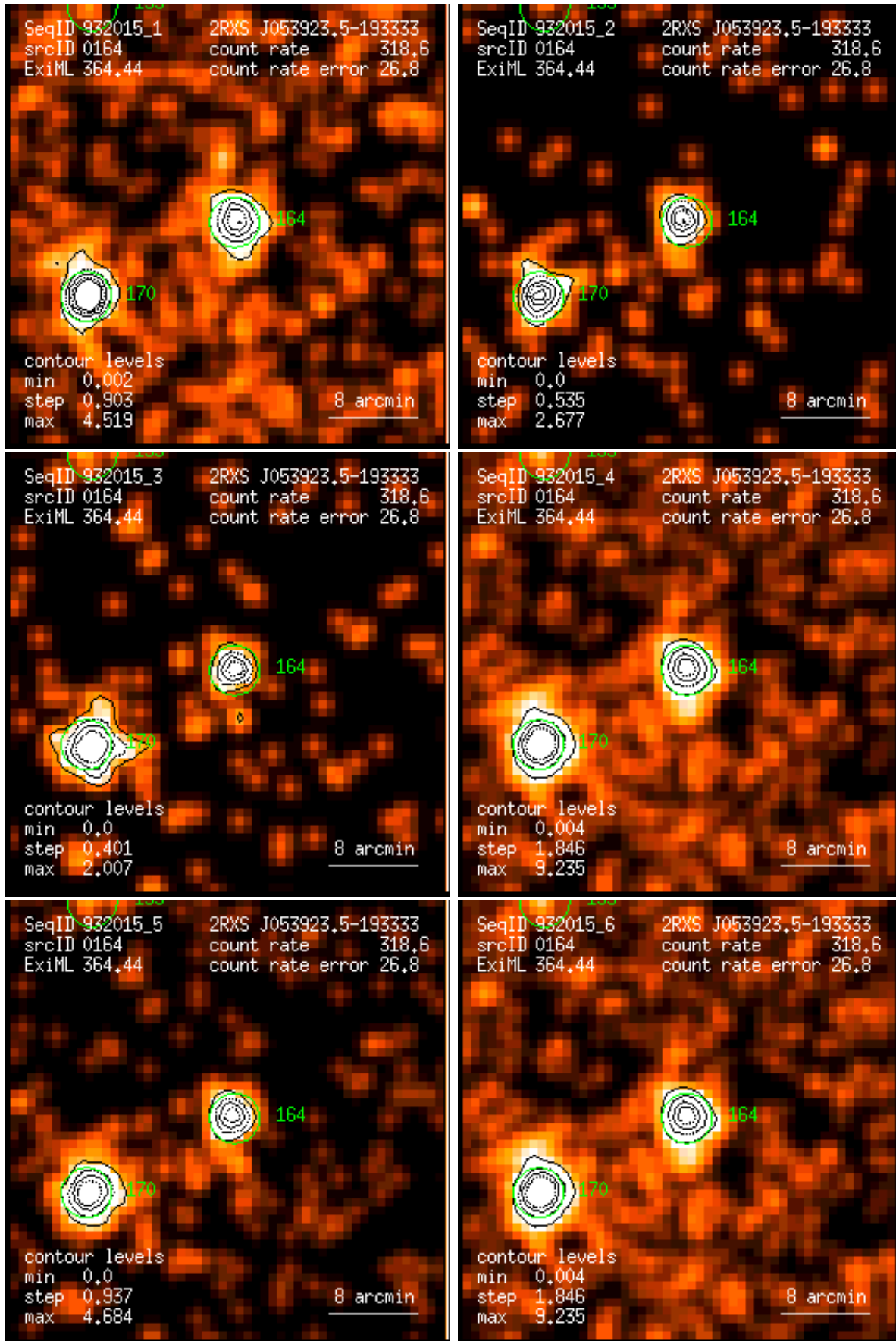
Figure 164: RASS 932015: detection 0164: band rate images, Gaussian filter: (1) PSPC channels 11 – 41, (2) 52 – 90, (3) 91 – 201, (4) 11 – 235, (5) 52 – 201, (6) 11 – 201. Broad band rates in counts/ks. Band rate contour levels in counts/ks/arcmin 2 .
