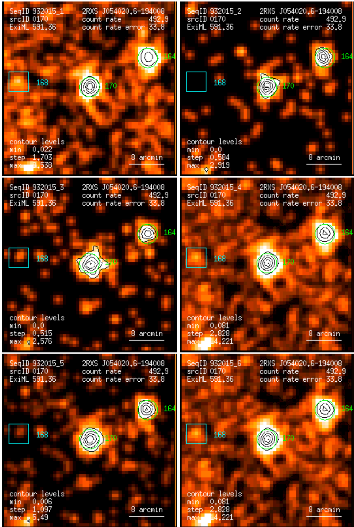
Figure 170: RASS 932015: detection 0170: band rate images, Gaussian filter: (1) PSPC channels 11 – 41, (2) 52 – 90, (3) 91 – 201, (4) 11 – 235, (5) 52 – 201, (6) 11 – 201. Broad band rates in counts/ks. Band rate contour levels in counts/ks/arcmin 2 .
