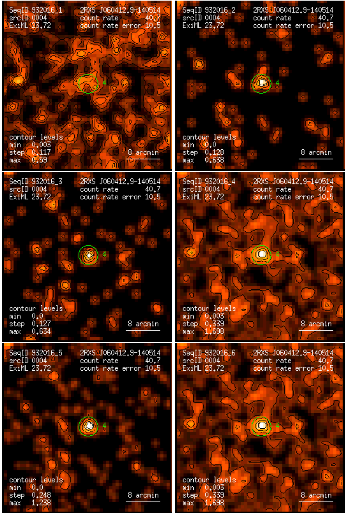
Figure 4: RASS 932016: detection 0004: band rate images, Gaussian filter: (1) PSPC channels 11 – 41, (2) 52 – 90, (3) 91 – 201, (4) 11 – 235, (5) 52 – 201, (6) 11 – 201. Broad band rates in counts/ks. Band rate contour levels in counts/ks/arcmin 2 .
