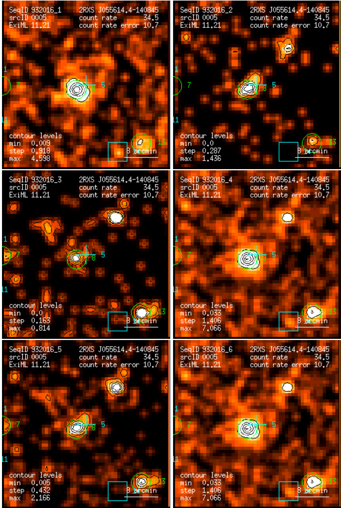
Figure 5: RASS 932016: detection 0005: band rate images, Gaussian filter: (1) PSPC channels 11 – 41, (2) 52 – 90, (3) 91 – 201, (4) 11 – 235, (5) 52 – 201, (6) 11 – 201. Broad band rates in counts/ks. Band rate contour levels in counts/ks/arcmin 2 .
