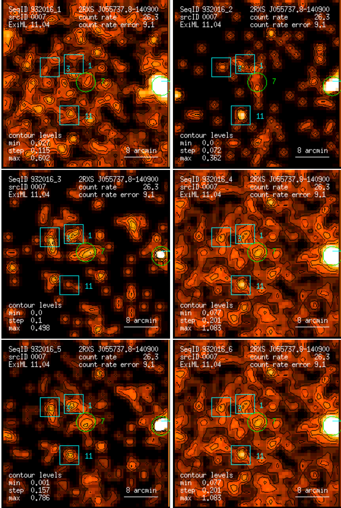
Figure 7: RASS 932016: detection 0007: band rate images, Gaussian filter: (1) PSPC channels 11 – 41, (2) 52 – 90, (3) 91 – 201, (4) 11 – 235, (5) 52 – 201, (6) 11 – 201. Broad band rates in counts/ks. Band rate contour levels in counts/ks/arcmin 2 .
