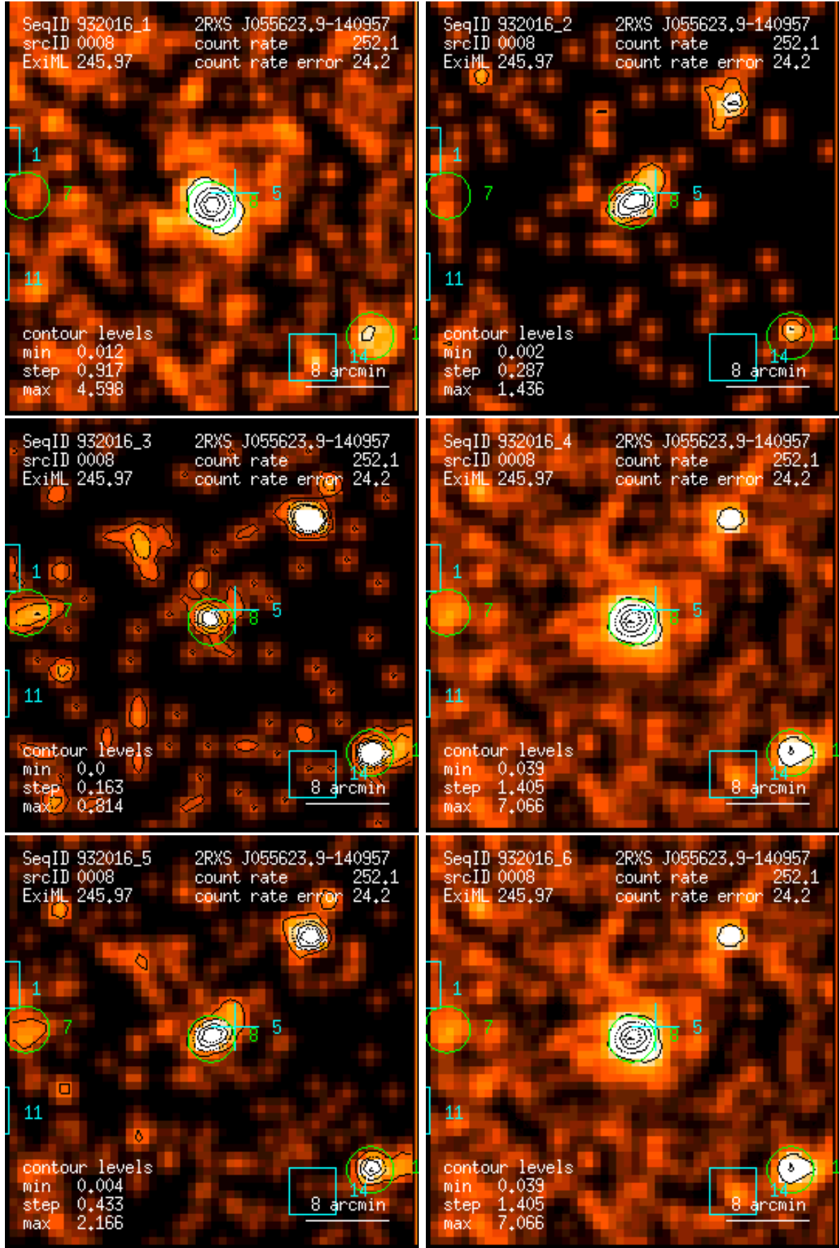
Figure 8: RASS 932016: detection 0008: band rate images, Gaussian filter: (1) PSPC channels 11 – 41, (2) 52 – 90, (3) 91 – 201, (4) 11 – 235, (5) 52 – 201, (6) 11 – 201. Broad band rates in counts/ks. Band rate contour levels in counts/ks/arcmin 2 .
