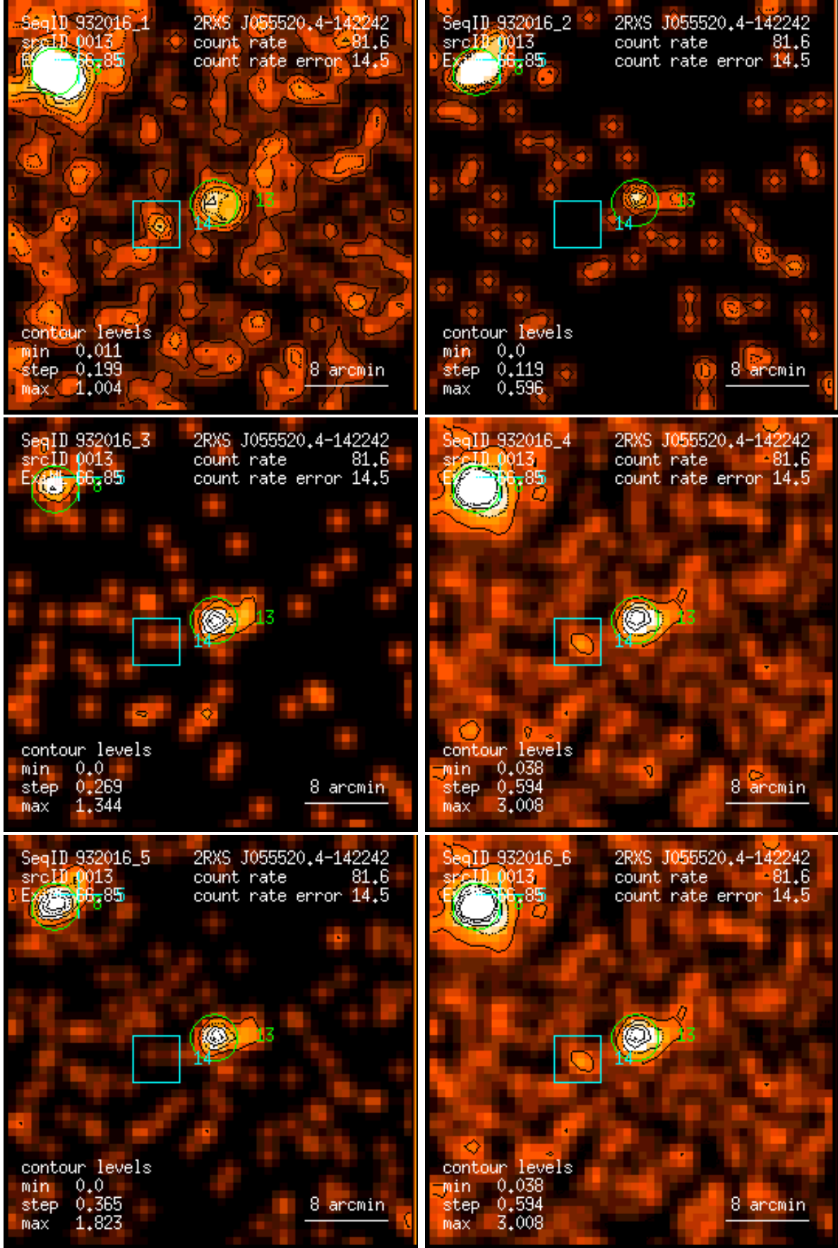
Figure 13: RASS 932016: detection 0013: band rate images, Gaussian filter: (1) PSPC channels 11 – 41, (2) 52 – 90, (3) 91 – 201, (4) 11 – 235, (5) 52 – 201, (6) 11 – 201. Broad band rates in counts/ks. Band rate contour levels in counts/ks/arcmin 2 .
