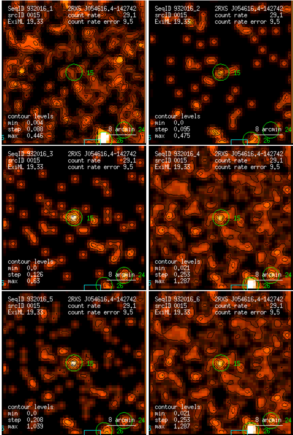
Figure 15: RASS 932016: detection 0015: band rate images, Gaussian filter: (1) PSPC channels 11 – 41, (2) 52 – 90, (3) 91 – 201, (4) 11 – 235, (5) 52 – 201, (6) 11 – 201. Broad band rates in counts/ks. Band rate contour levels in counts/ks/arcmin 2 .
