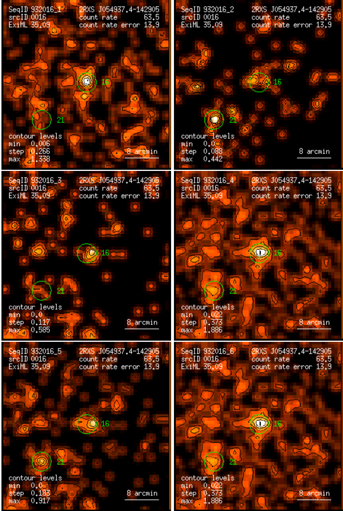
Figure 16: RASS 932016: detection 0016: band rate images, Gaussian filter: (1) PSPC channels 11 – 41, (2) 52 – 90, (3) 91 – 201, (4) 11 – 235, (5) 52 – 201, (6) 11 – 201. Broad band rates in counts/ks. Band rate contour levels in counts/ks/arcmin 2 .
