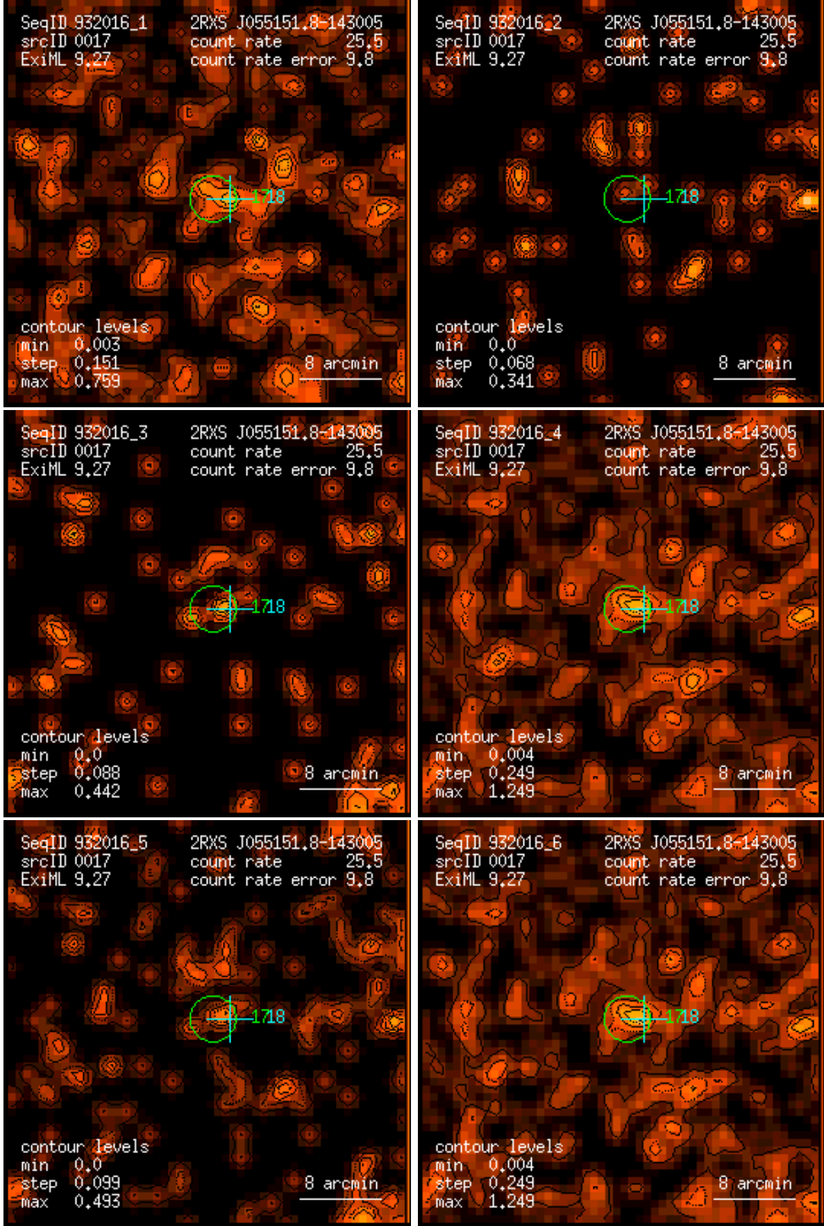
Figure 17: RASS 932016: detection 0017: band rate images, Gaussian filter: (1) PSPC channels 11 – 41, (2) 52 – 90, (3) 91 – 201, (4) 11 – 235, (5) 52 – 201, (6) 11 – 201. Broad band rates in counts/ks. Band rate contour levels in counts/ks/arcmin 2 .
