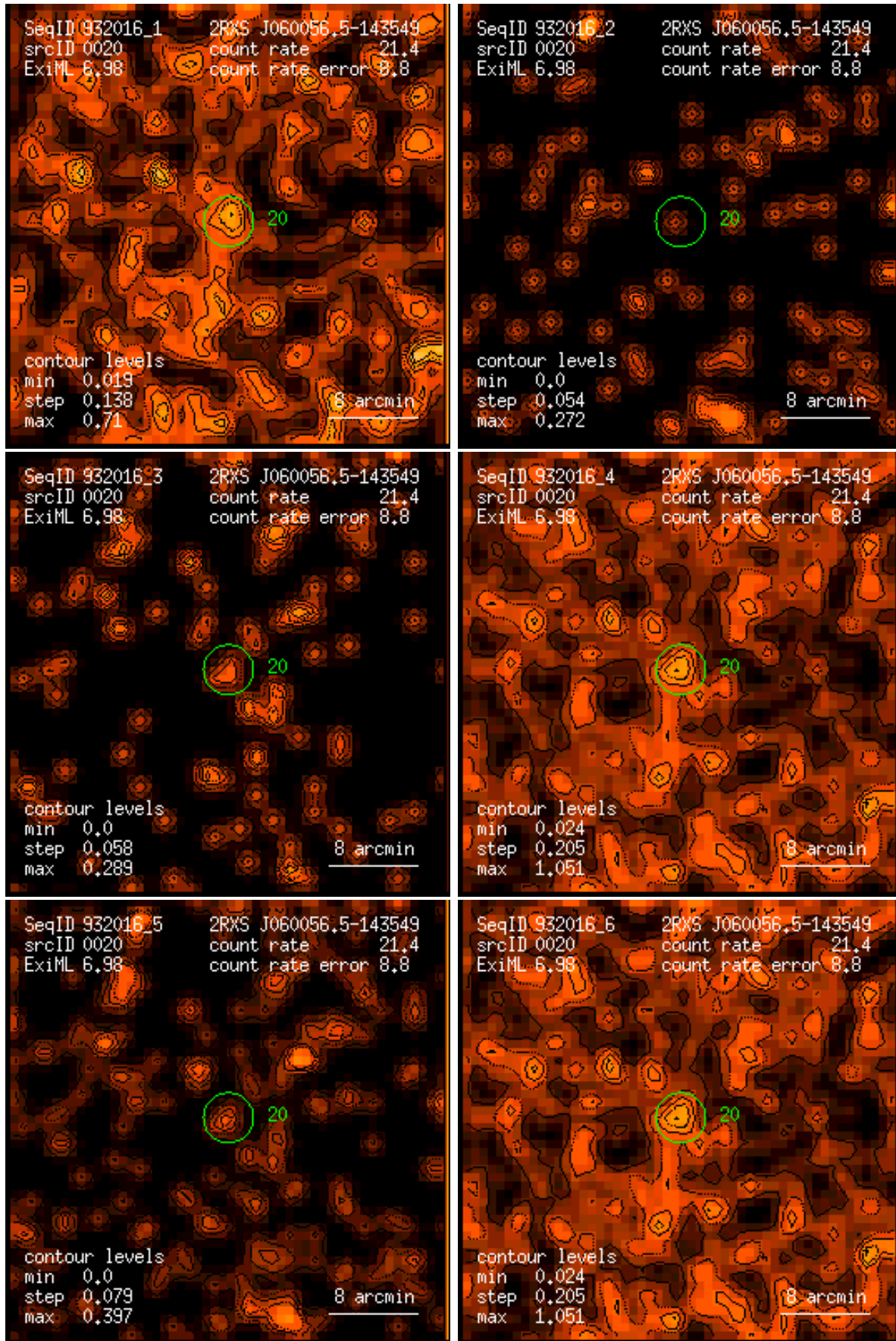
Figure 20: RASS 932016: detection 0020: band rate images, Gaussian filter: (1) PSPC channels 11 – 41, (2) 52 – 90, (3) 91 – 201, (4) 11 – 235, (5) 52 – 201, (6) 11 – 201. Broad band rates in counts/ks. Band rate contour levels in counts/ks/arcmin 2 .
