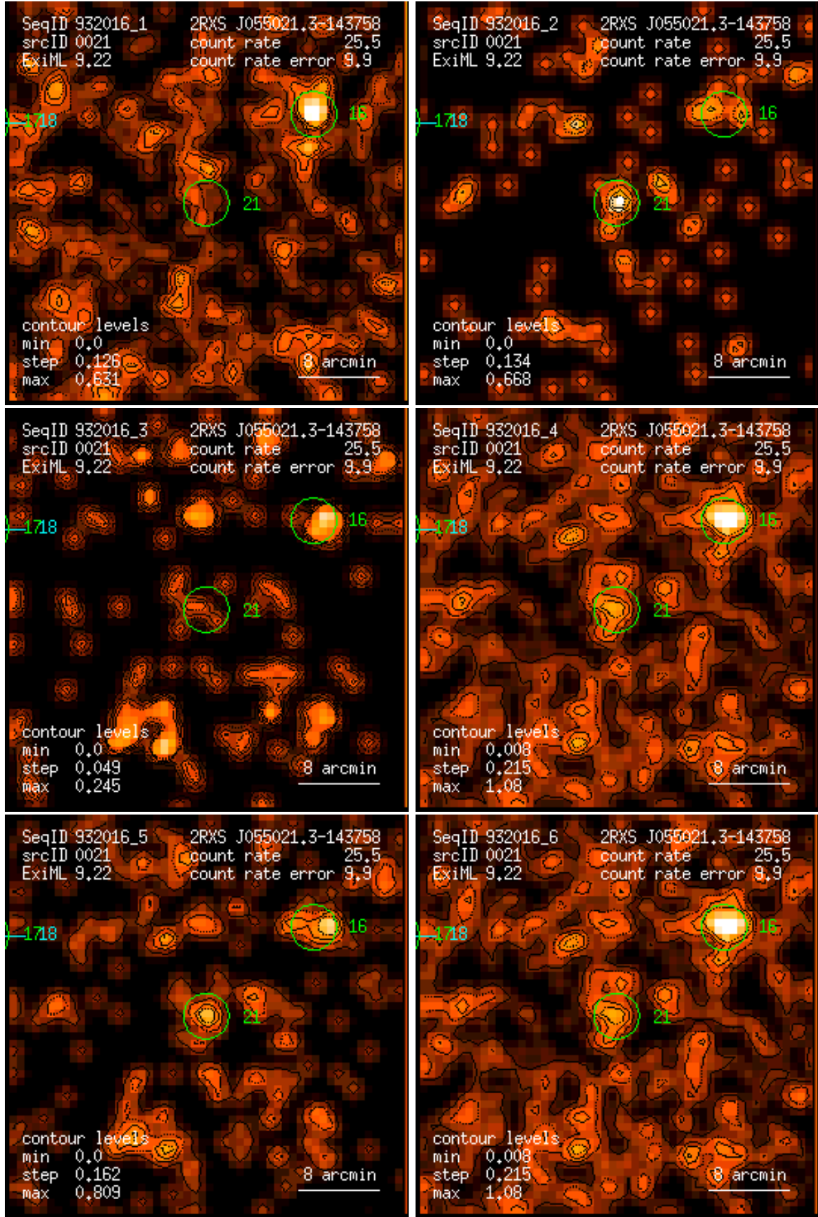
Figure 21: RASS 932016: detection 0021: band rate images, Gaussian filter: (1) PSPC channels 11 – 41, (2) 52 – 90, (3) 91 – 201, (4) 11 – 235, (5) 52 – 201, (6) 11 – 201. Broad band rates in counts/ks. Band rate contour levels in counts/ks/arcmin 2 .
