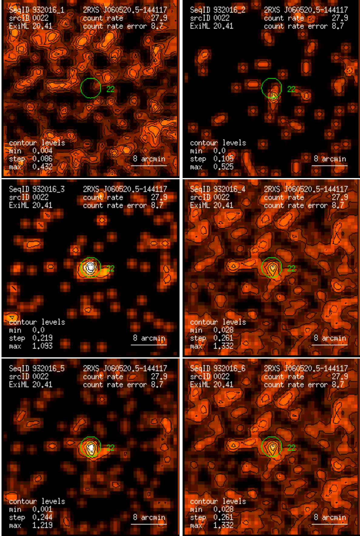
Figure 22: RASS 932016: detection 0022: band rate images, Gaussian filter: (1) PSPC channels 11 – 41, (2) 52 – 90, (3) 91 – 201, (4) 11 – 235, (5) 52 – 201, (6) 11 – 201. Broad band rates in counts/ks. Band rate contour levels in counts/ks/arcmin 2 .
