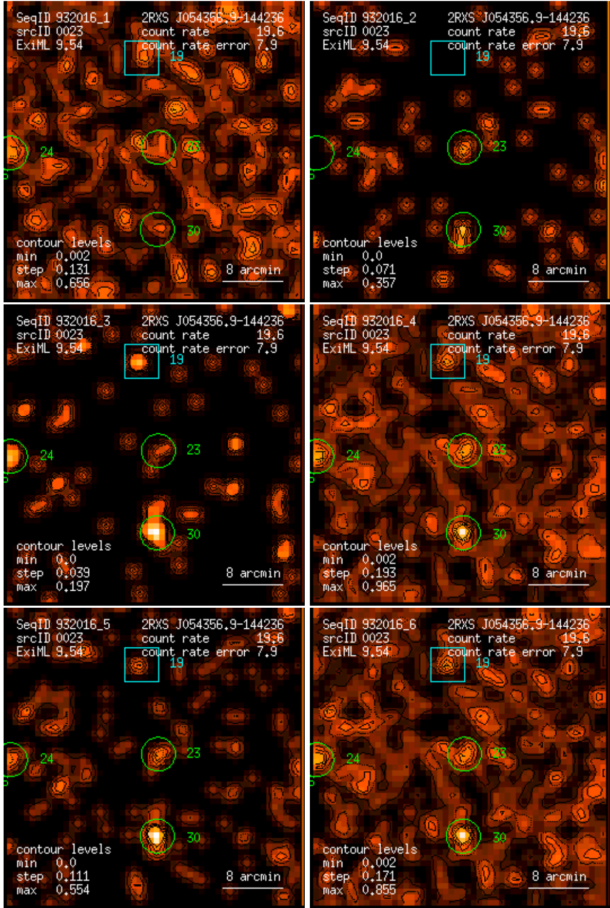
Figure 23: RASS 932016: detection 0023: band rate images, Gaussian filter: (1) PSPC channels 11 – 41, (2) 52 – 90, (3) 91 – 201, (4) 11 – 235, (5) 52 – 201, (6) 11 – 201. Broad band rates in counts/ks. Band rate contour levels in counts/ks/arcmin 2 .
