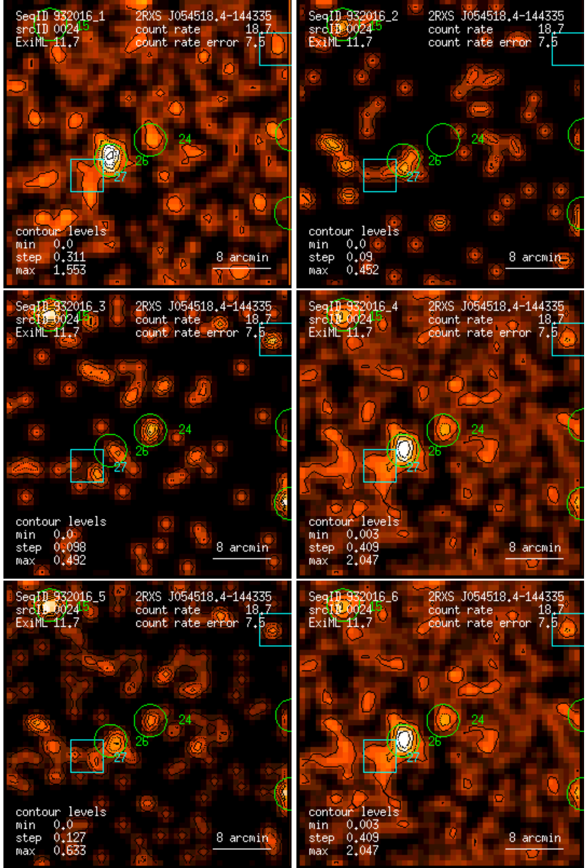
Figure 24: RASS 932016: detection 0024: band rate images, Gaussian filter: (1) PSPC channels 11 – 41, (2) 52 – 90, (3) 91 – 201, (4) 11 – 235, (5) 52 – 201, (6) 11 – 201. Broad band rates in counts/ks. Band rate contour levels in counts/ks/arcmin 2 .
