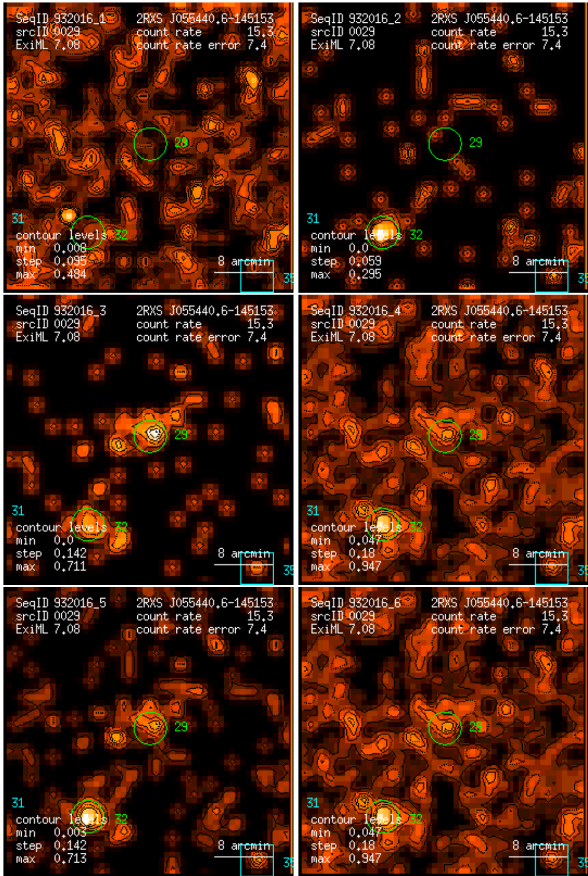
Figure 29: RASS 932016: detection 0029: band rate images, Gaussian filter: (1) PSPC channels 11 – 41, (2) 52 – 90, (3) 91 – 201, (4) 11 – 235, (5) 52 – 201, (6) 11 – 201. Broad band rates in counts/ks. Band rate contour levels in counts/ks/arcmin 2 .
