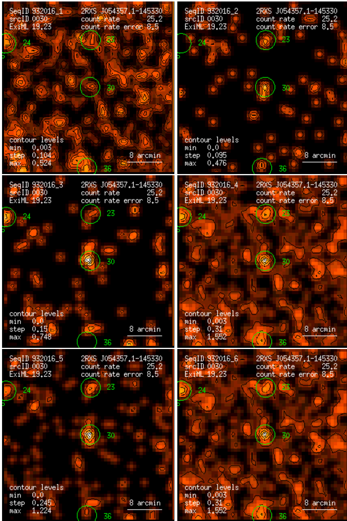
Figure 30: RASS 932016: detection 0030: band rate images, Gaussian filter: (1) PSPC channels 11 – 41, (2) 52 – 90, (3) 91 – 201, (4) 11 – 235, (5) 52 – 201, (6) 11 – 201. Broad band rates in counts/ks. Band rate contour levels in counts/ks/arcmin 2 .
