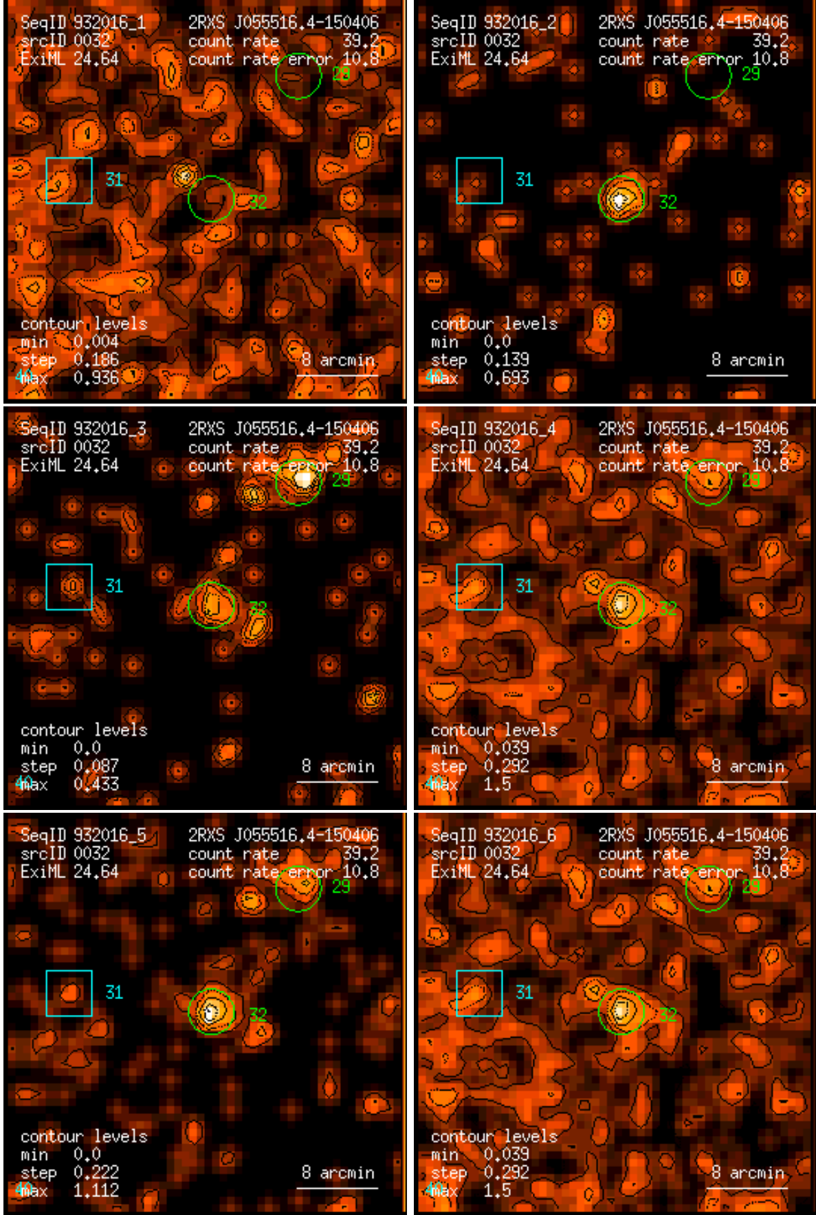
Figure 32: RASS 932016: detection 0032: band rate images, Gaussian filter: (1) PSPC channels 11 – 41, (2) 52 – 90, (3) 91 – 201, (4) 11 – 235, (5) 52 – 201, (6) 11 – 201. Broad band rates in counts/ks. Band rate contour levels in counts/ks/arcmin 2 .
