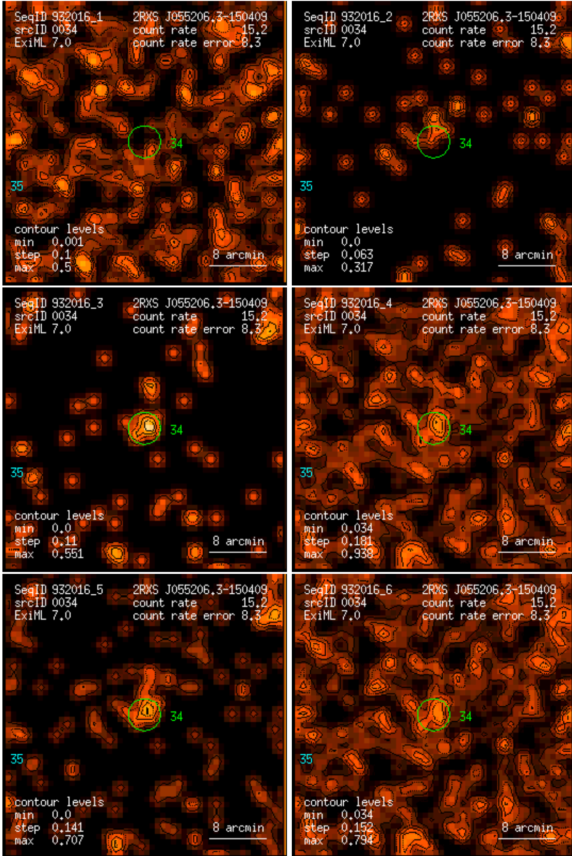
Figure 34: RASS 932016: detection 0034: band rate images, Gaussian filter: (1) PSPC channels 11 – 41, (2) 52 – 90, (3) 91 – 201, (4) 11 – 235, (5) 52 – 201, (6) 11 – 201. Broad band rates in counts/ks. Band rate contour levels in counts/ks/arcmin 2 .
