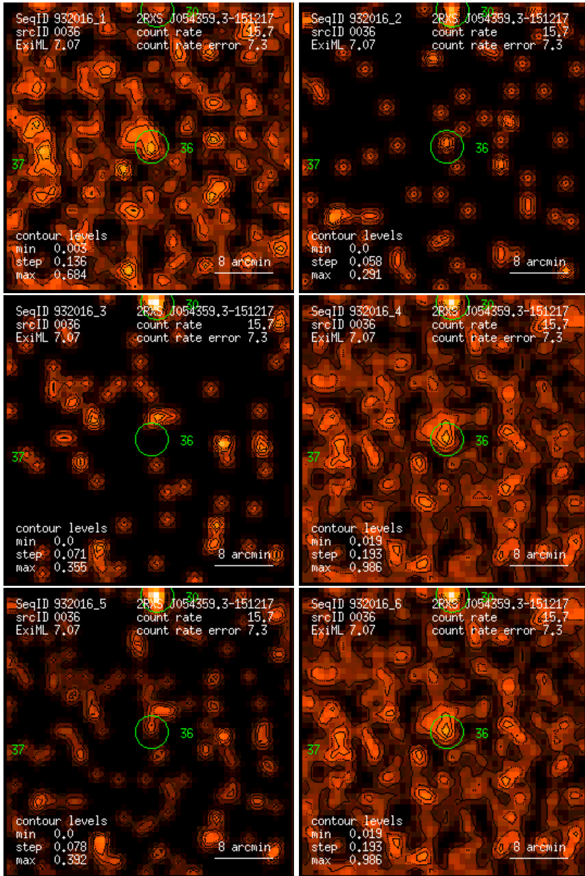
Figure 36: RASS 932016: detection 0036: band rate images, Gaussian filter: (1) PSPC channels 11 – 41, (2) 52 – 90, (3) 91 – 201, (4) 11 – 235, (5) 52 – 201, (6) 11 – 201. Broad band rates in counts/ks. Band rate contour levels in counts/ks/arcmin 2 .
