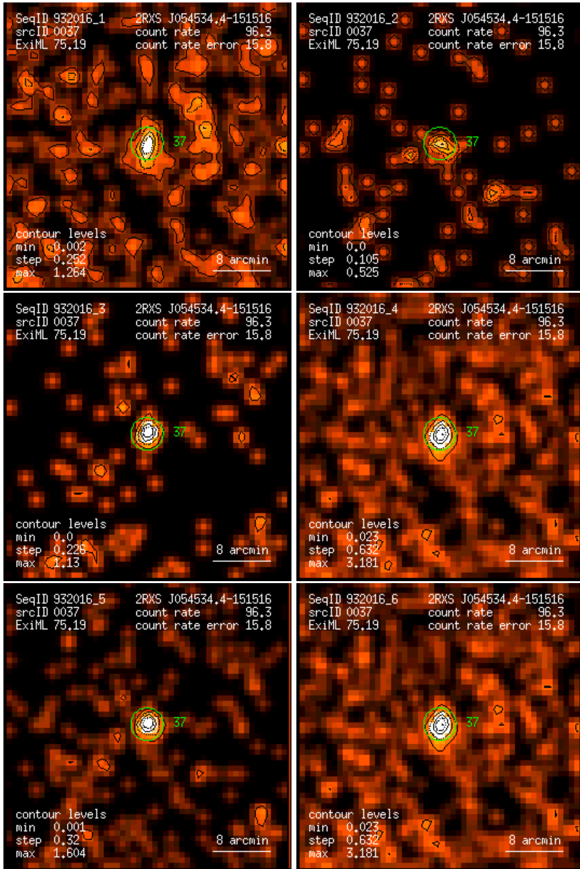
Figure 37: RASS 932016: detection 0037: band rate images, Gaussian filter: (1) PSPC channels 11 – 41, (2) 52 – 90, (3) 91 – 201, (4) 11 – 235, (5) 52 – 201, (6) 11 – 201. Broad band rates in counts/ks. Band rate contour levels in counts/ks/arcmin 2 .
