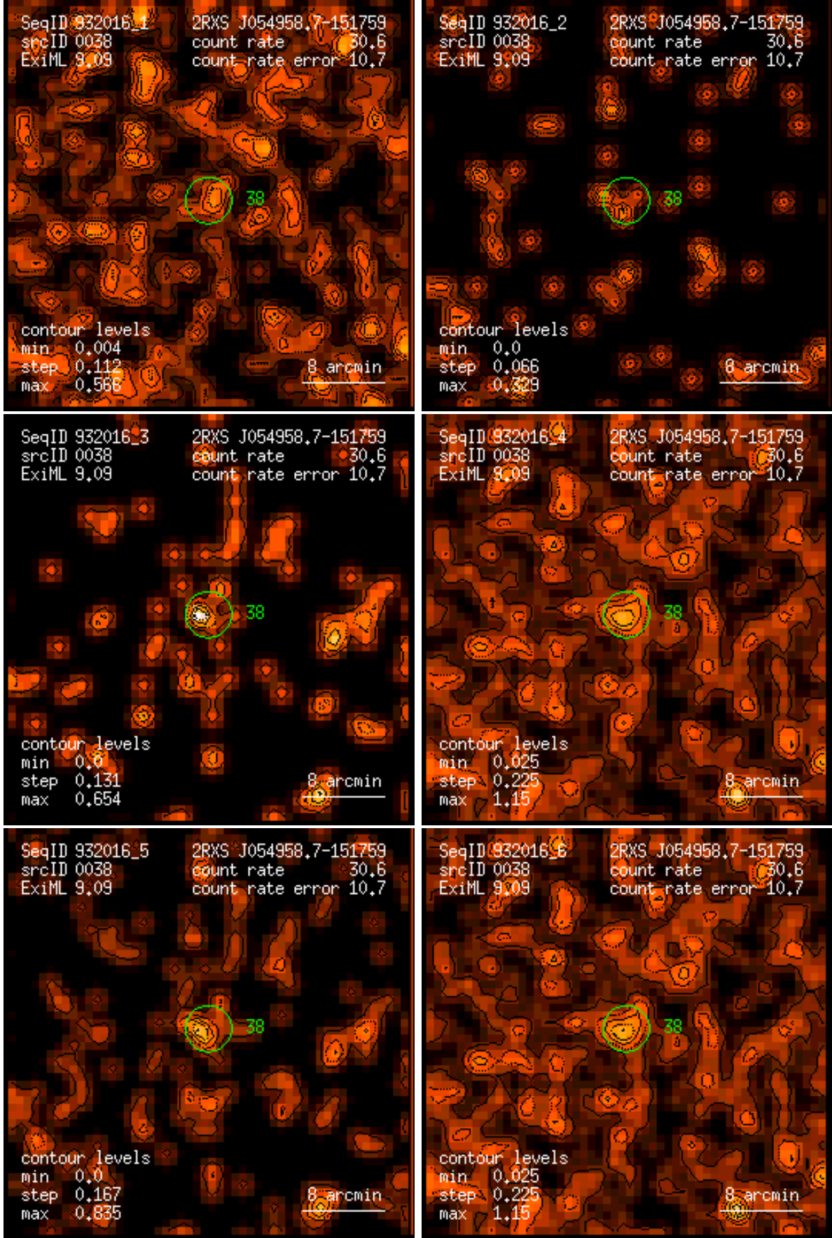
Figure 38: RASS 932016: detection 0038: band rate images, Gaussian filter: (1) PSPC channels 11 – 41, (2) 52 – 90, (3) 91 – 201, (4) 11 – 235, (5) 52 – 201, (6) 11 – 201. Broad band rates in counts/ks. Band rate contour levels in counts/ks/arcmin 2 .
