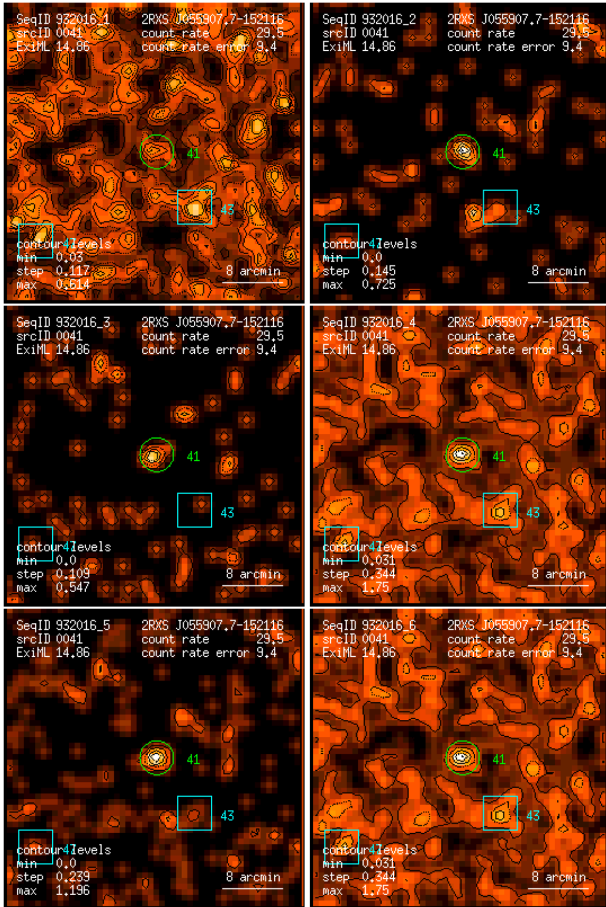
Figure 41: RASS 932016: detection 0041: band rate images, Gaussian filter: (1) PSPC channels 11 – 41, (2) 52 – 90, (3) 91 – 201, (4) 11 – 235, (5) 52 – 201, (6) 11 – 201. Broad band rates in counts/ks. Band rate contour levels in counts/ks/arcmin 2 .
