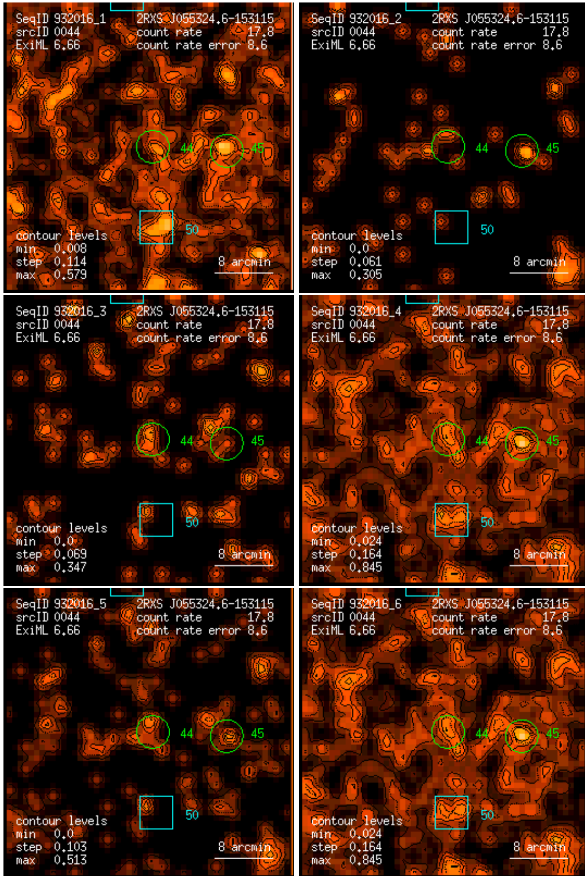
Figure 44: RASS 932016: detection 0044: band rate images, Gaussian filter: (1) PSPC channels 11 – 41, (2) 52 – 90, (3) 91 – 201, (4) 11 – 235, (5) 52 – 201, (6) 11 – 201. Broad band rates in counts/ks. Band rate contour levels in counts/ks/arcmin 2 .
