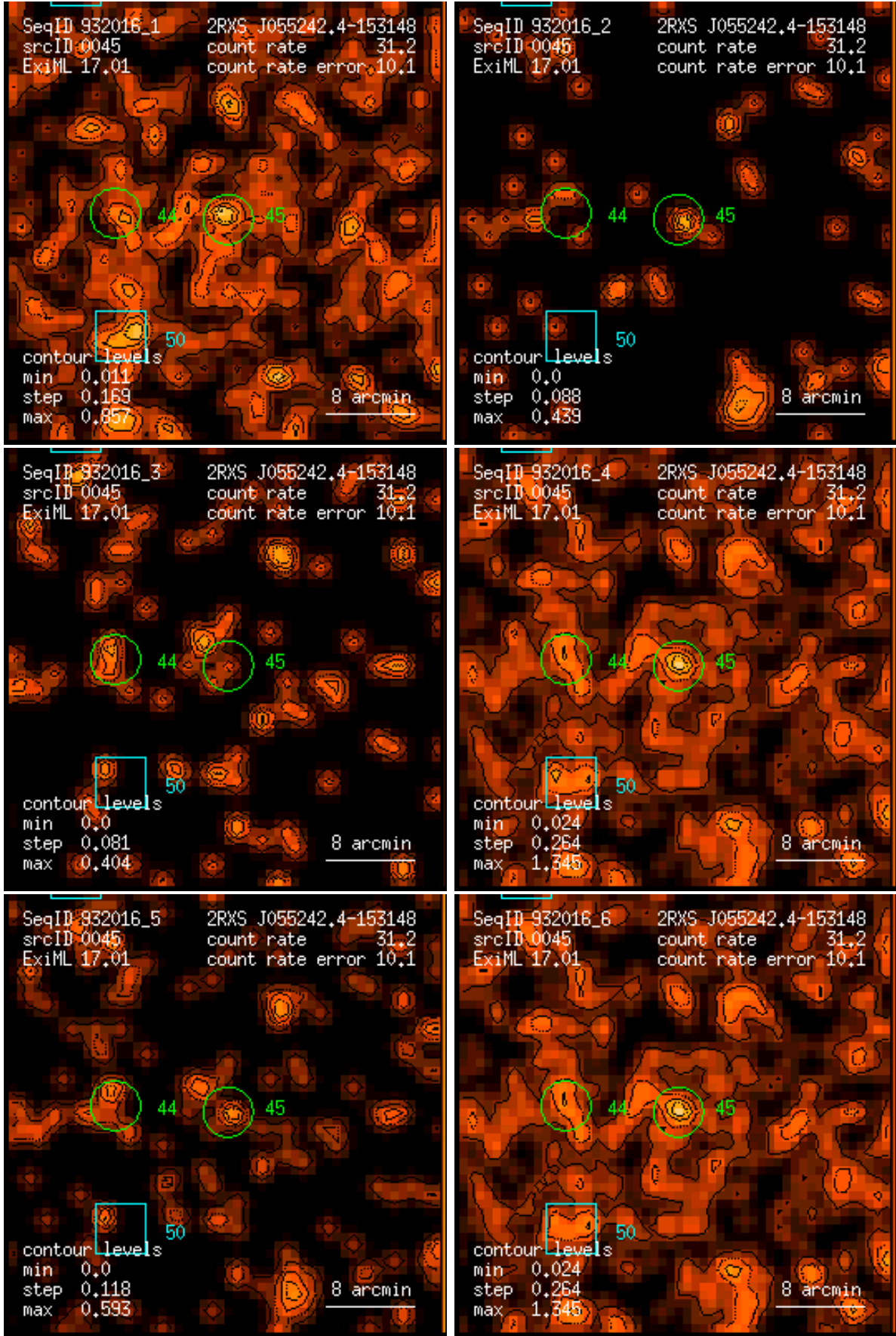
Figure 45: RASS 932016: detection 0045: band rate images, Gaussian filter: (1) PSPC channels 11 – 41, (2) 52 – 90, (3) 91 – 201, (4) 11 – 235, (5) 52 – 201, (6) 11 – 201. Broad band rates in counts/ks. Band rate contour levels in counts/ks/arcmin 2 .
