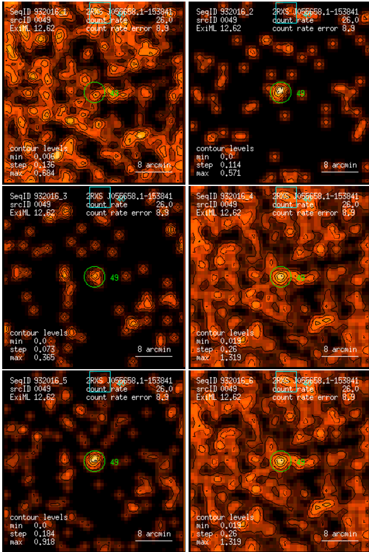
Figure 49: RASS 932016: detection 0049: band rate images, Gaussian filter: (1) PSPC channels 11 – 41, (2) 52 – 90, (3) 91 – 201, (4) 11 – 235, (5) 52 – 201, (6) 11 – 201. Broad band rates in counts/ks. Band rate contour levels in counts/ks/arcmin 2 .
