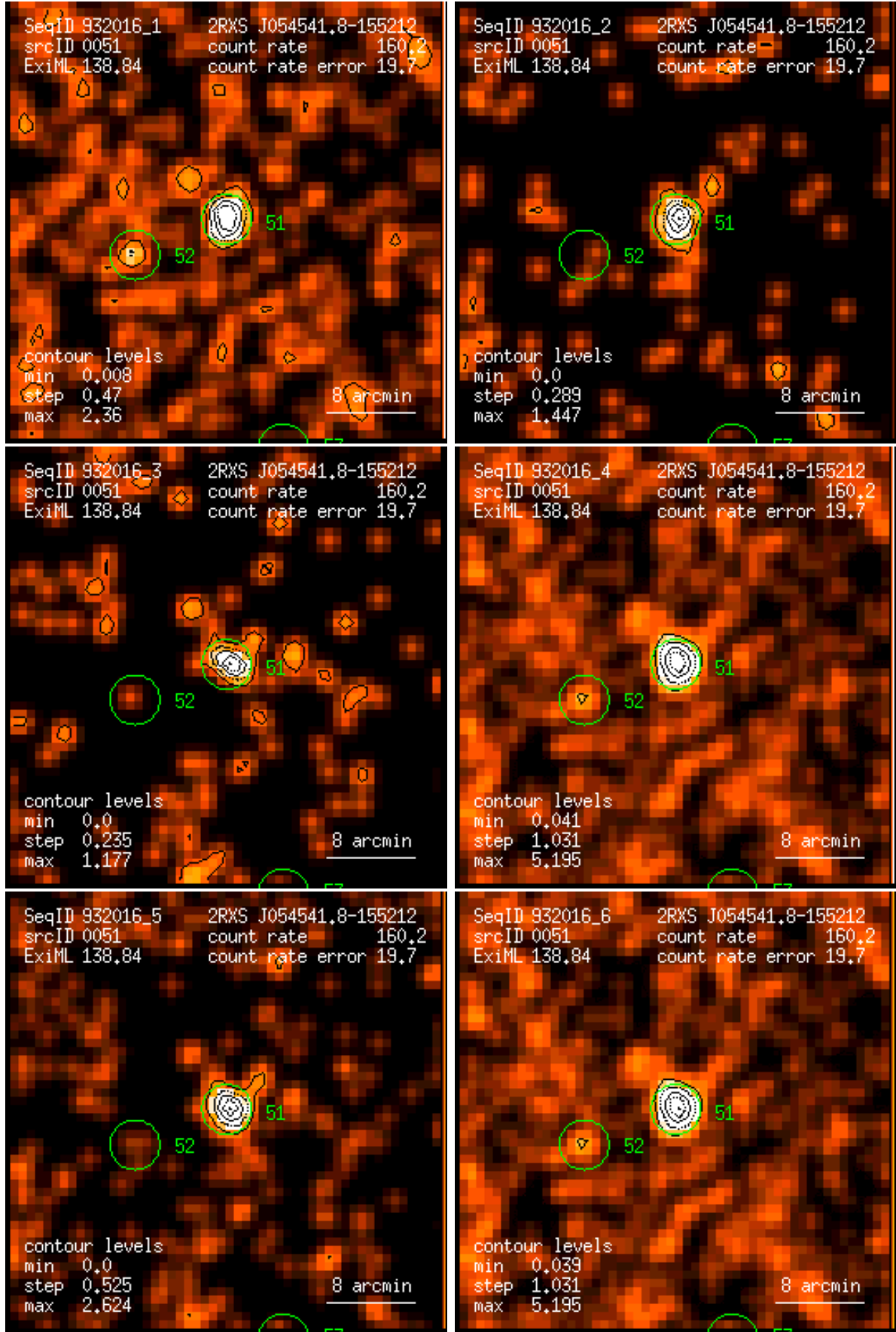
Figure 51: RASS 932016: detection 0051: band rate images, Gaussian filter: (1) PSPC channels 11 – 41, (2) 52 – 90, (3) 91 – 201, (4) 11 – 235, (5) 52 – 201, (6) 11 – 201. Broad band rates in counts/ks. Band rate contour levels in counts/ks/arcmin 2 .
