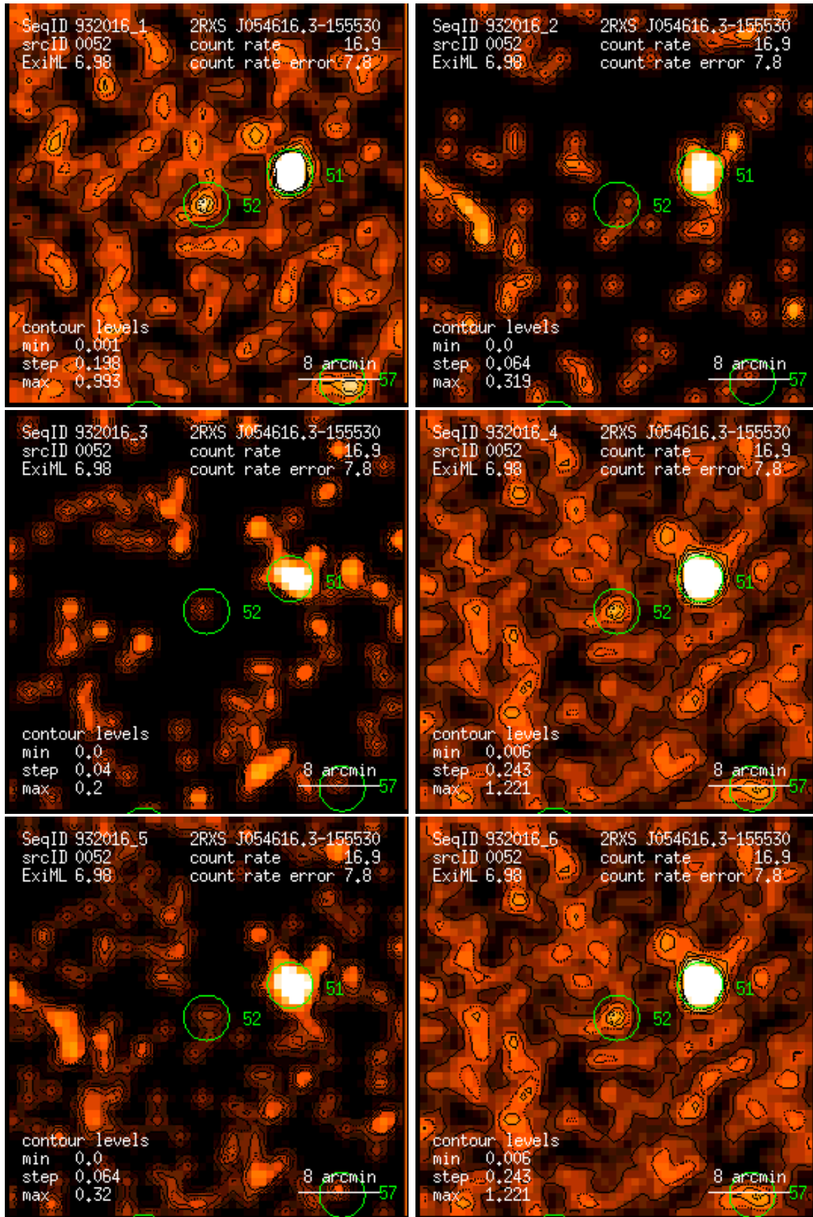
Figure 52: RASS 932016: detection 0052: band rate images, Gaussian filter: (1) PSPC channels 11 – 41, (2) 52 – 90, (3) 91 – 201, (4) 11 – 235, (5) 52 – 201, (6) 11 – 201. Broad band rates in counts/ks. Band rate contour levels in counts/ks/arcmin 2 .
