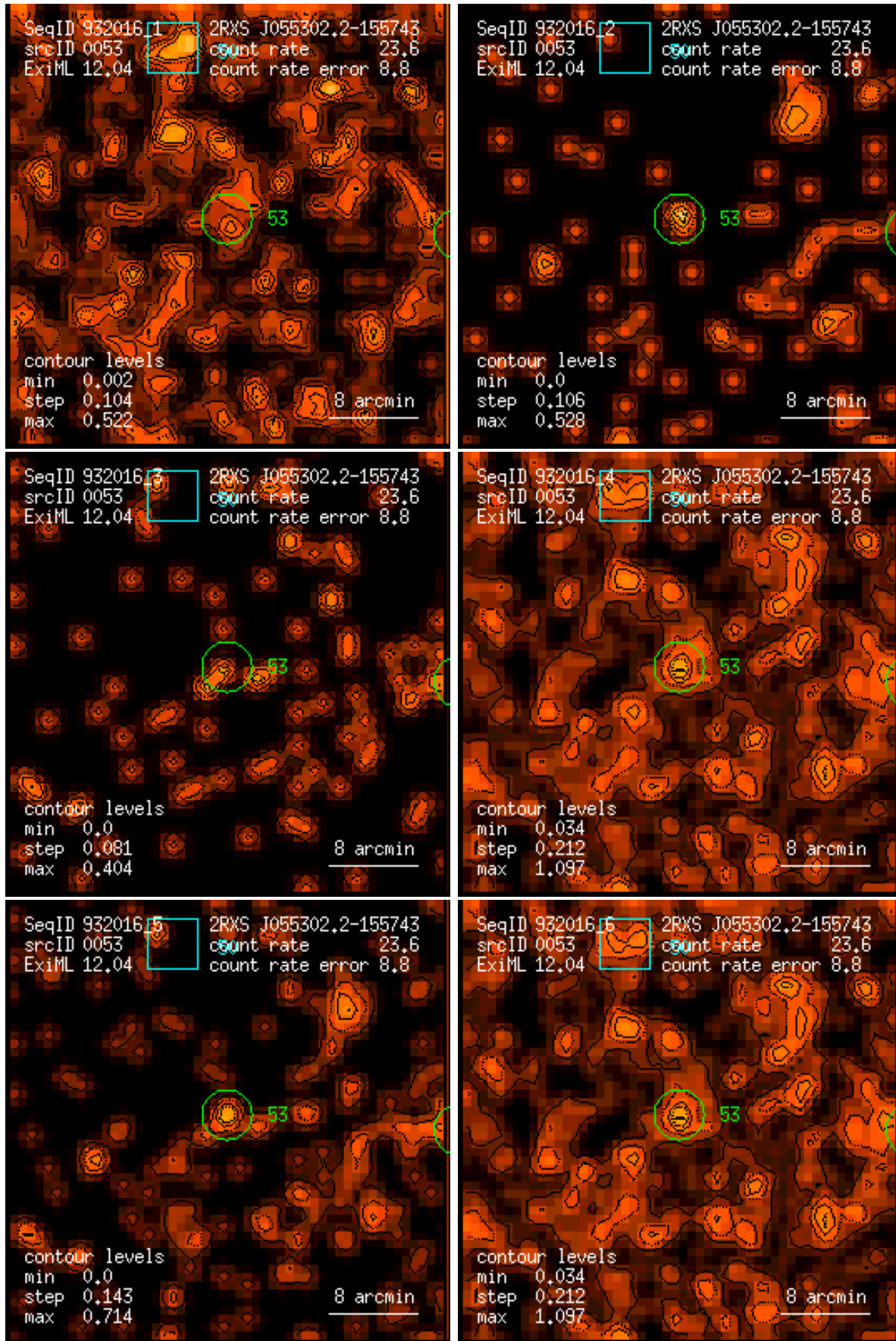
Figure 53: RASS 932016: detection 0053: band rate images, Gaussian filter: (1) PSPC channels 11 – 41, (2) 52 – 90, (3) 91 – 201, (4) 11 – 235, (5) 52 – 201, (6) 11 – 201. Broad band rates in counts/ks. Band rate contour levels in counts/ks/arcmin 2 .
