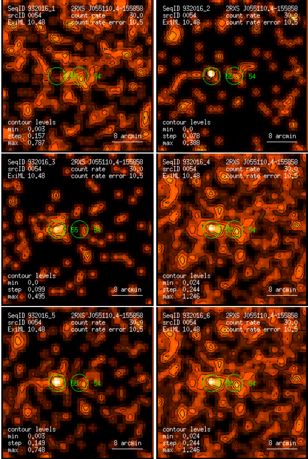
Figure 54: RASS 932016: detection 0054: band rate images, Gaussian filter: (1) PSPC channels 11 – 41, (2) 52 – 90, (3) 91 – 201, (4) 11 – 235, (5) 52 – 201, (6) 11 – 201. Broad band rates in counts/ks. Band rate contour levels in counts/ks/arcmin 2 .
