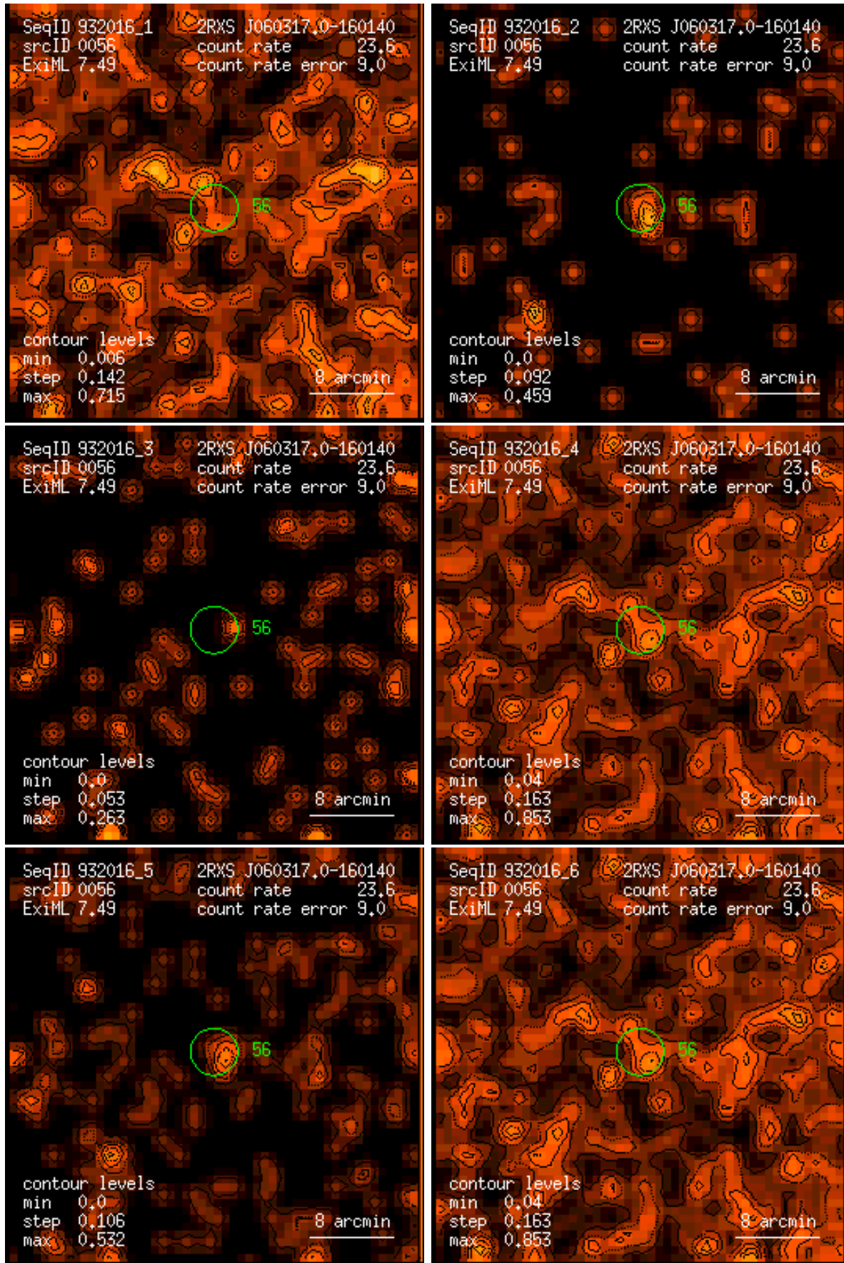
Figure 56: RASS 932016: detection 0056: band rate images, Gaussian filter: (1) PSPC channels 11 – 41, (2) 52 – 90, (3) 91 – 201, (4) 11 – 235, (5) 52 – 201, (6) 11 – 201. Broad band rates in counts/ks. Band rate contour levels in counts/ks/arcmin 2 .
