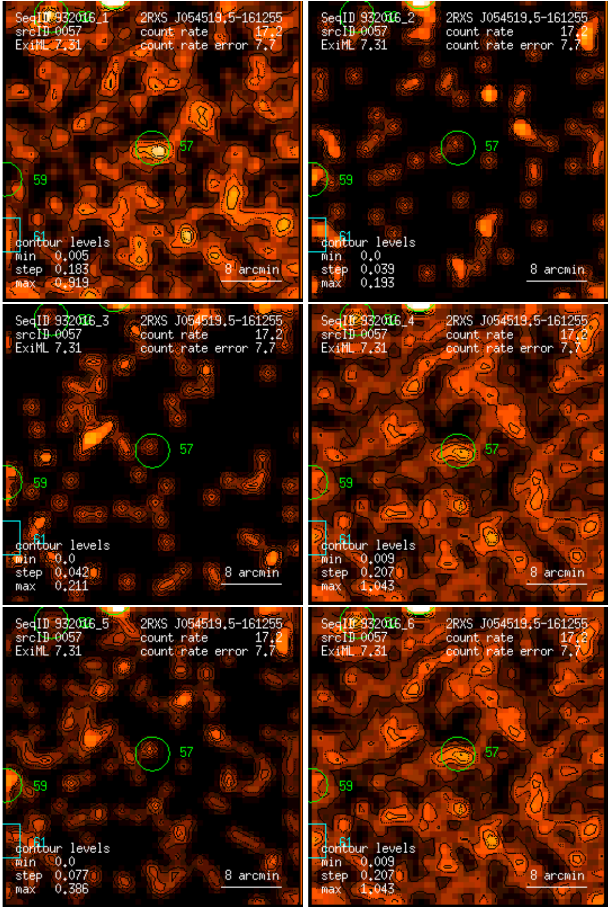
Figure 57: RASS 932016: detection 0057: band rate images, Gaussian filter: (1) PSPC channels 11 – 41, (2) 52 – 90, (3) 91 – 201, (4) 11 – 235, (5) 52 – 201, (6) 11 – 201. Broad band rates in counts/ks. Band rate contour levels in counts/ks/arcmin 2 .
