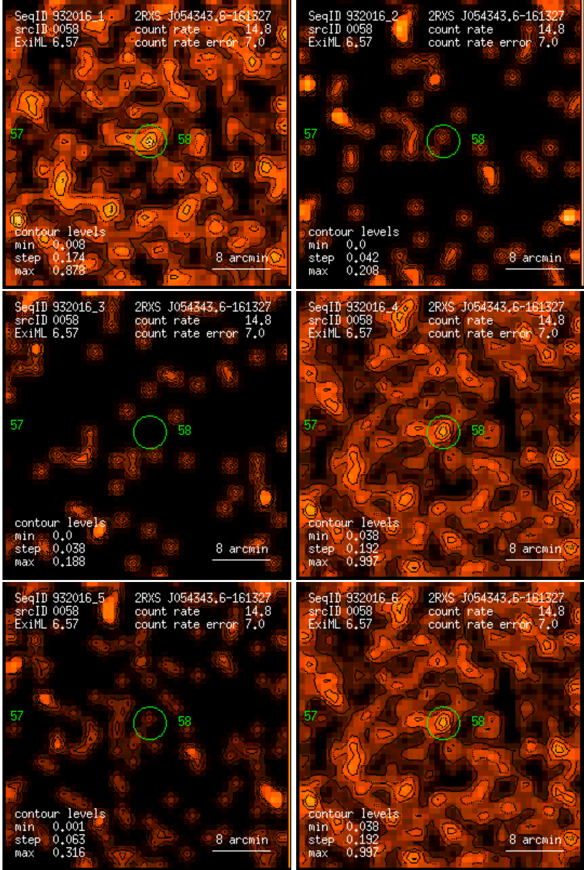
Figure 58: RASS 932016: detection 0058: band rate images, Gaussian filter: (1) PSPC channels 11 – 41, (2) 52 – 90, (3) 91 – 201, (4) 11 – 235, (5) 52 – 201, (6) 11 – 201. Broad band rates in counts/ks. Band rate contour levels in counts/ks/arcmin 2 .
