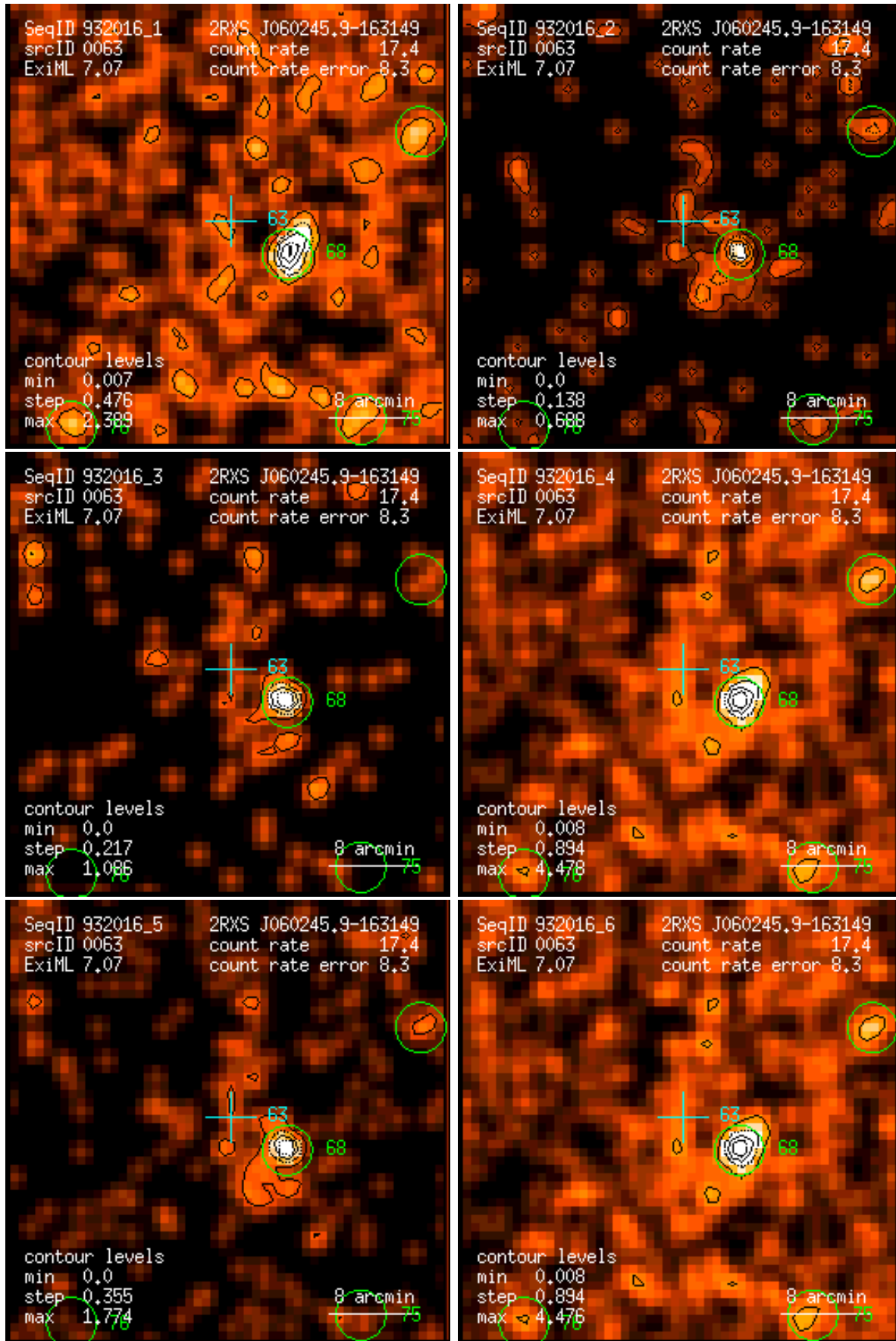
Figure 63: RASS 932016: detection 0063: band rate images, Gaussian filter: (1) PSPC channels 11 – 41, (2) 52 – 90, (3) 91 – 201, (4) 11 – 235, (5) 52 – 201, (6) 11 – 201. Broad band rates in counts/ks. Band rate contour levels in counts/ks/arcmin 2 .
