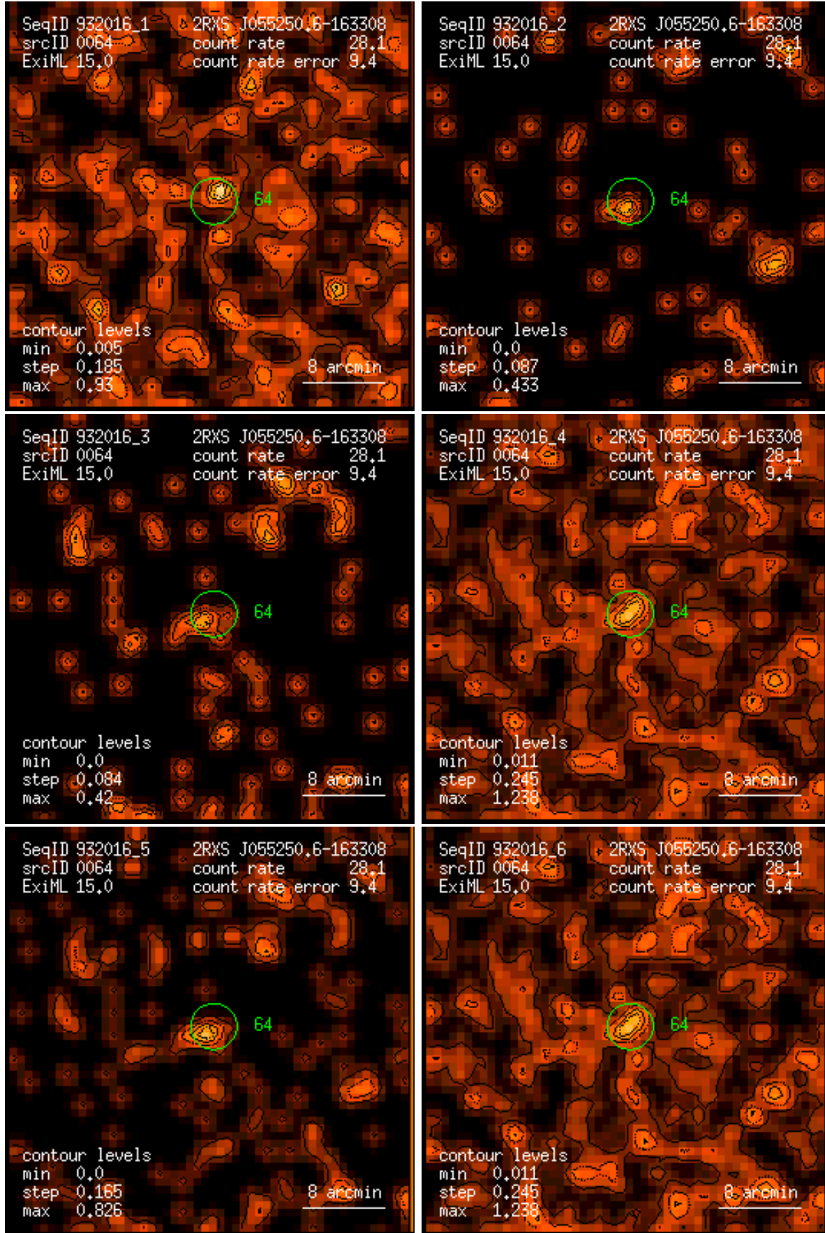
Figure 64: RASS 932016: detection 0064: band rate images, Gaussian filter: (1) PSPC channels 11 – 41, (2) 52 – 90, (3) 91 – 201, (4) 11 – 235, (5) 52 – 201, (6) 11 – 201. Broad band rates in counts/ks. Band rate contour levels in counts/ks/arcmin 2 .
