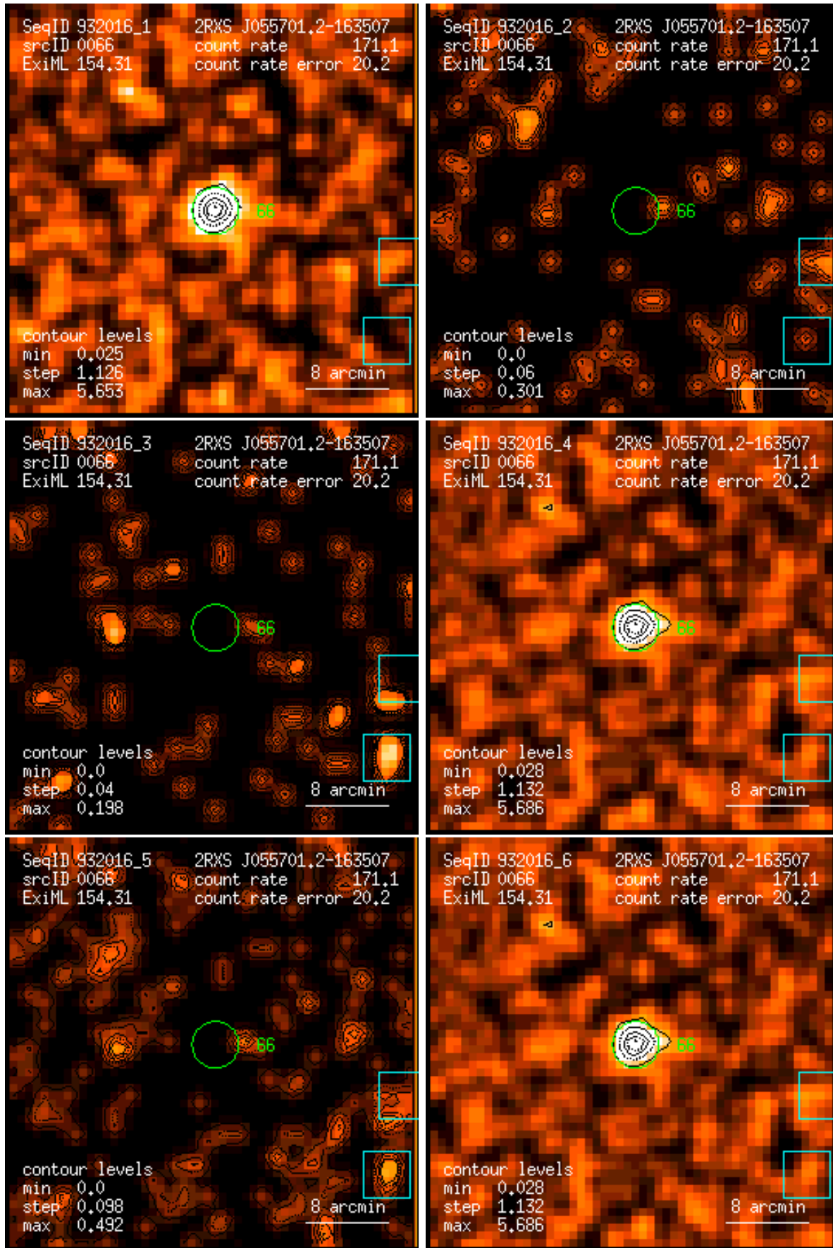
Figure 66: RASS 932016: detection 0066: band rate images, Gaussian filter: (1) PSPC channels 11 – 41, (2) 52 – 90, (3) 91 – 201, (4) 11 – 235, (5) 52 – 201, (6) 11 – 201. Broad band rates in counts/ks. Band rate contour levels in counts/ks/arcmin 2 .
