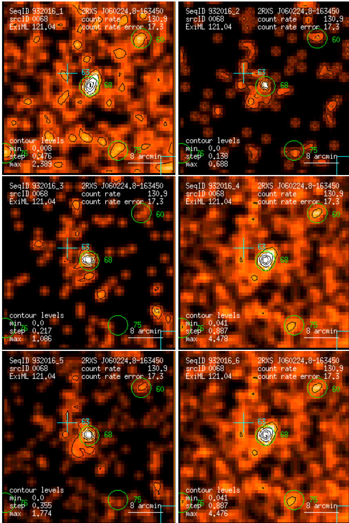
Figure 68: RASS 932016: detection 0068: band rate images, Gaussian filter: (1) PSPC channels 11 – 41, (2) 52 – 90, (3) 91 – 201, (4) 11 – 235, (5) 52 – 201, (6) 11 – 201. Broad band rates in counts/ks. Band rate contour levels in counts/ks/arcmin 2 .
