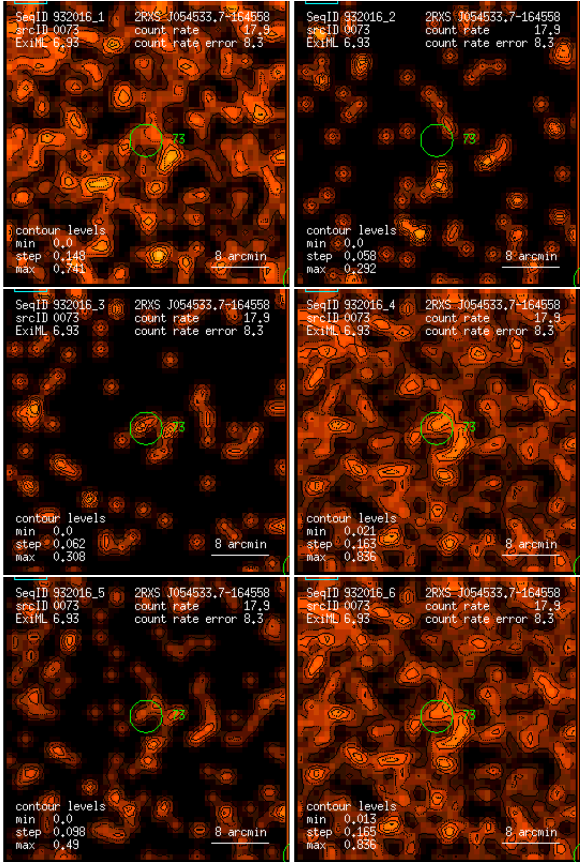
Figure 73: RASS 932016: detection 0073: band rate images, Gaussian filter: (1) PSPC channels 11 – 41, (2) 52 – 90, (3) 91 – 201, (4) 11 – 235, (5) 52 – 201, (6) 11 – 201. Broad band rates in counts/ks. Band rate contour levels in counts/ks/arcmin 2 .
