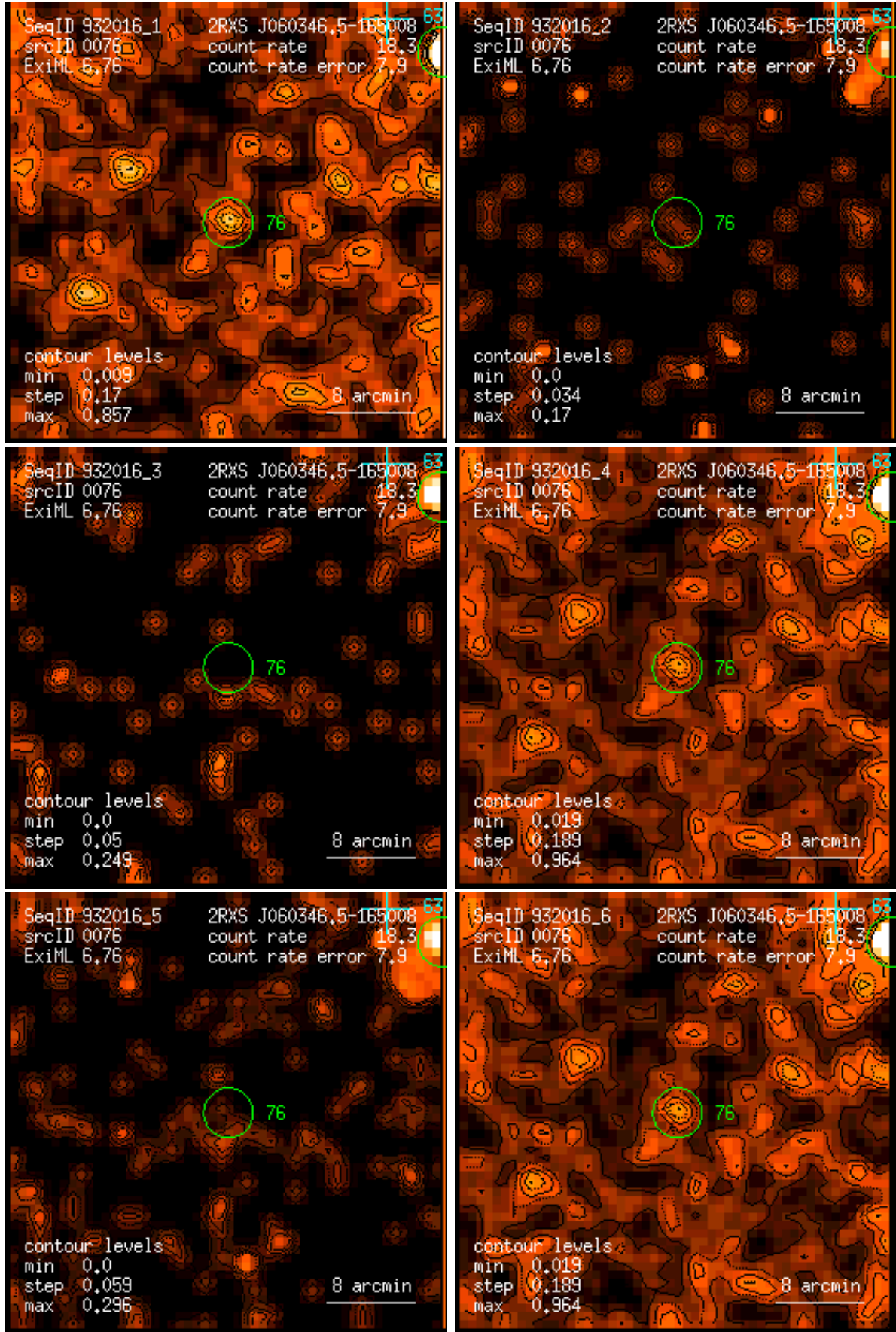
Figure 76: RASS 932016: detection 0076: band rate images, Gaussian filter: (1) PSPC channels 11 – 41, (2) 52 – 90, (3) 91 – 201, (4) 11 – 235, (5) 52 – 201, (6) 11 – 201. Broad band rates in counts/ks. Band rate contour levels in counts/ks/arcmin 2 .
