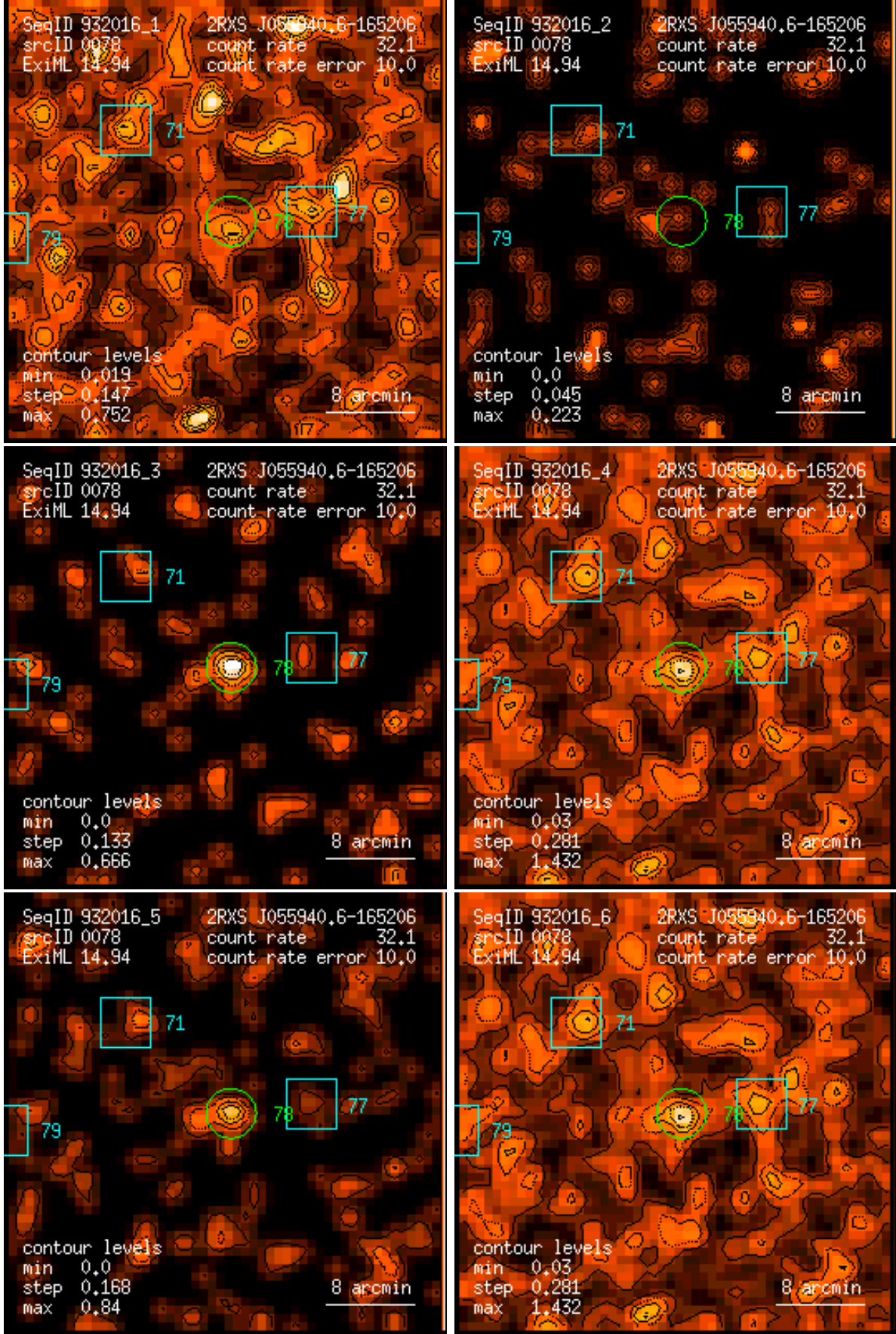
Figure 78: RASS 932016: detection 0078: band rate images, Gaussian filter: (1) PSPC channels 11 – 41, (2) 52 – 90, (3) 91 – 201, (4) 11 – 235, (5) 52 – 201, (6) 11 – 201. Broad band rates in counts/ks. Band rate contour levels in counts/ks/arcmin 2 .
