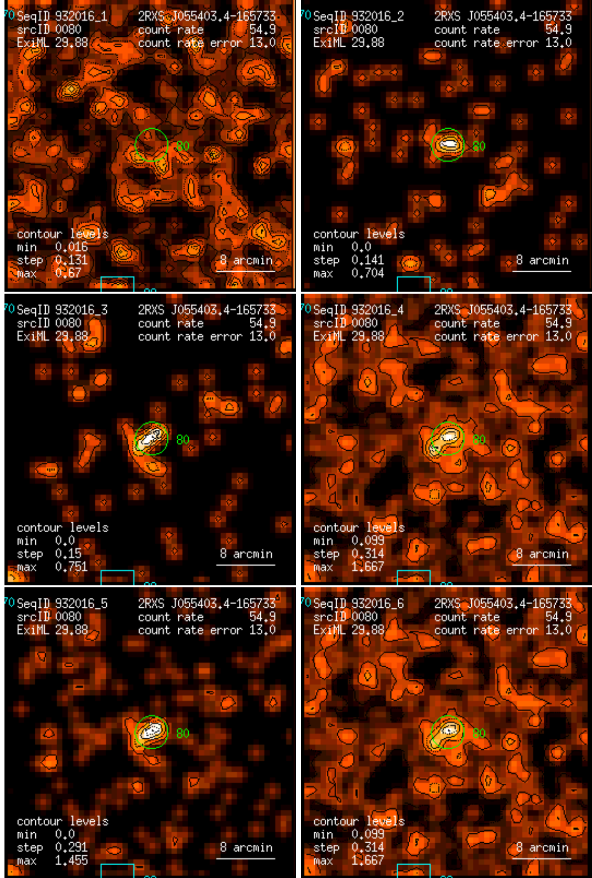
Figure 80: RASS 932016: detection 0080: band rate images, Gaussian filter: (1) PSPC channels 11 – 41, (2) 52 – 90, (3) 91 – 201, (4) 11 – 235, (5) 52 – 201, (6) 11 – 201. Broad band rates in counts/ks. Band rate contour levels in counts/ks/arcmin 2 .
