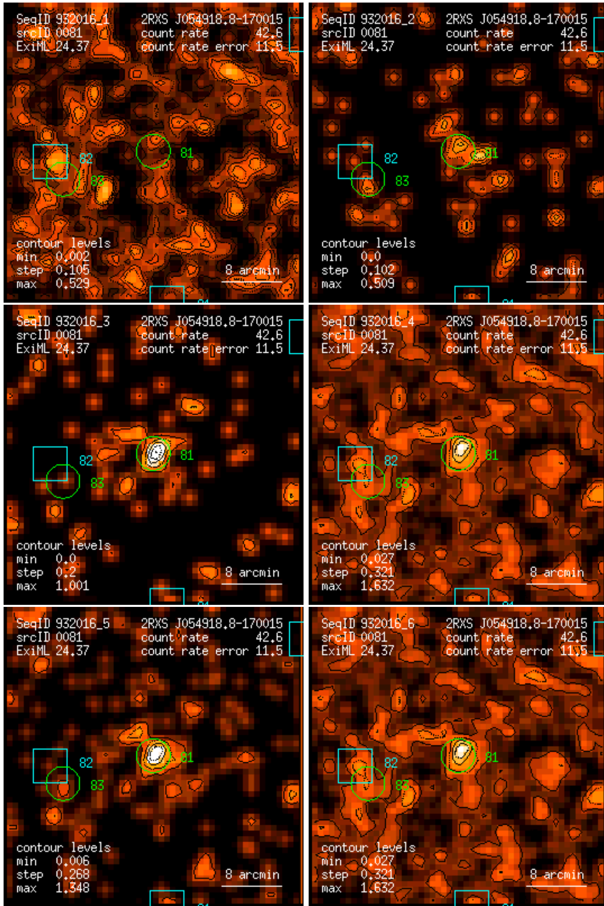
Figure 81: RASS 932016: detection 0081: band rate images, Gaussian filter: (1) PSPC channels 11 – 41, (2) 52 – 90, (3) 91 – 201, (4) 11 – 235, (5) 52 – 201, (6) 11 – 201. Broad band rates in counts/ks. Band rate contour levels in counts/ks/arcmin 2 .
