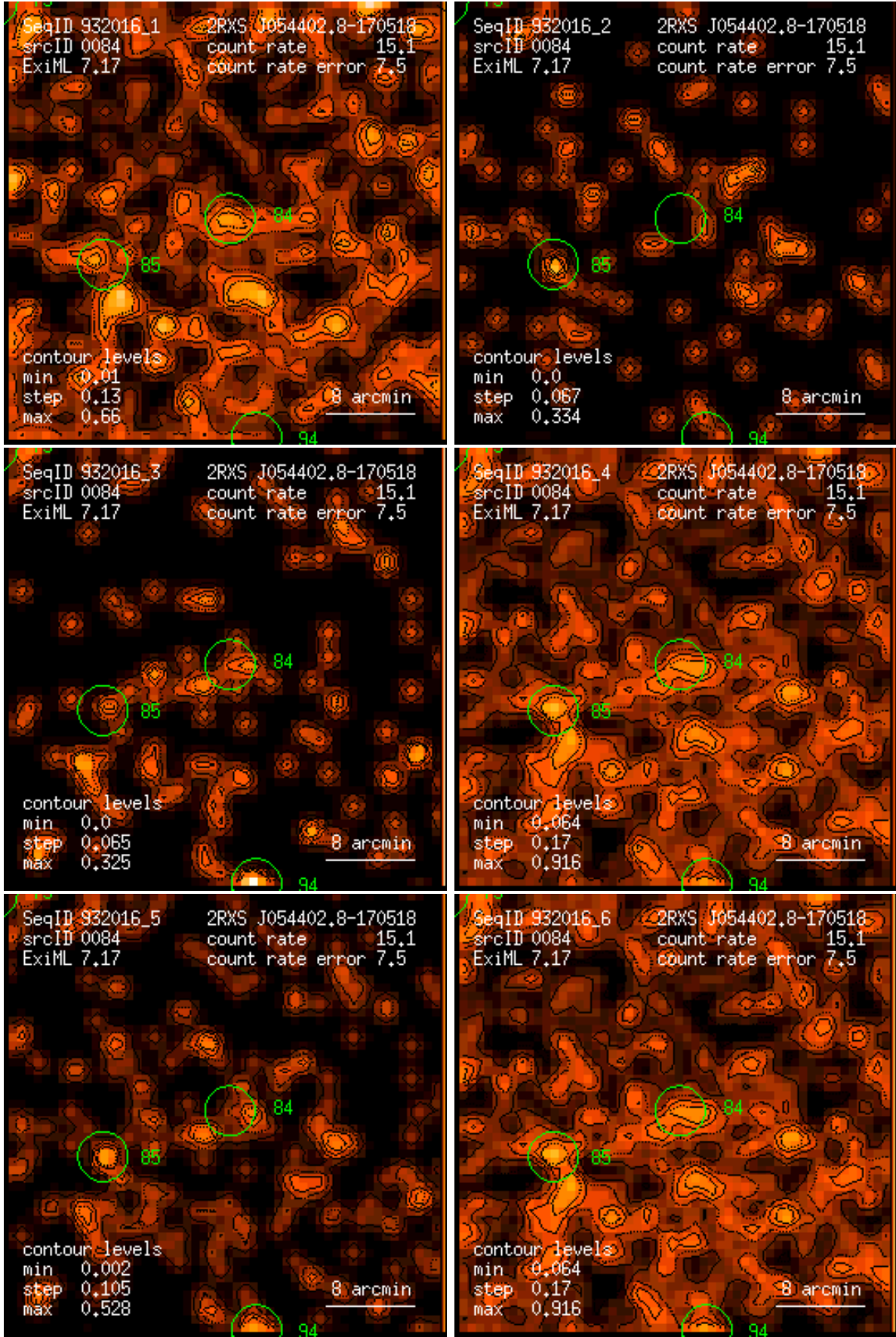
Figure 84: RASS 932016: detection 0084: band rate images, Gaussian filter: (1) PSPC channels 11 – 41, (2) 52 – 90, (3) 91 – 201, (4) 11 – 235, (5) 52 – 201, (6) 11 – 201. Broad band rates in counts/ks. Band rate contour levels in counts/ks/arcmin 2 .
