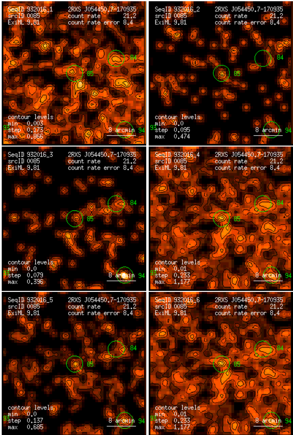
Figure 85: RASS 932016: detection 0085: band rate images, Gaussian filter: (1) PSPC channels 11 – 41, (2) 52 – 90, (3) 91 – 201, (4) 11 – 235, (5) 52 – 201, (6) 11 – 201. Broad band rates in counts/ks. Band rate contour levels in counts/ks/arcmin 2 .
