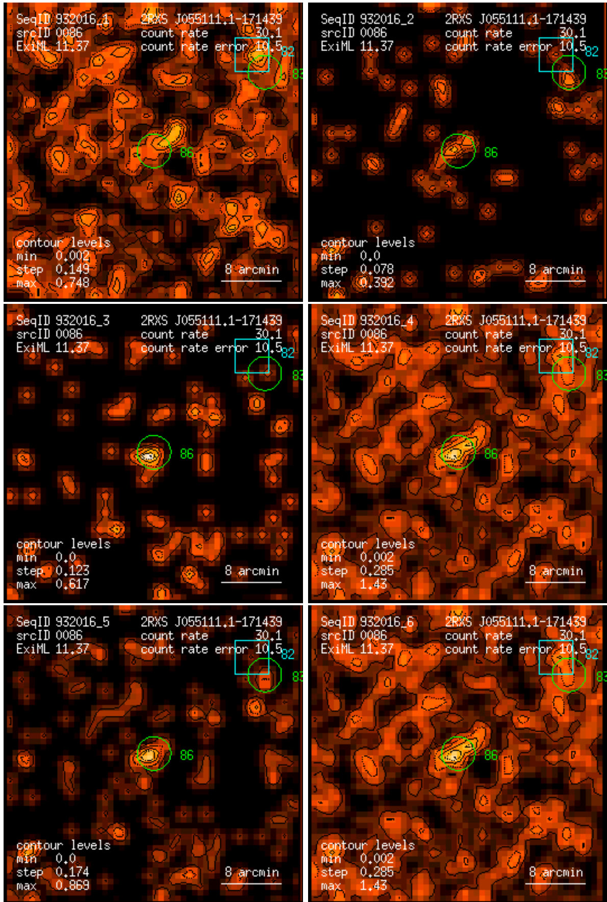
Figure 86: RASS 932016: detection 0086: band rate images, Gaussian filter: (1) PSPC channels 11 – 41, (2) 52 – 90, (3) 91 – 201, (4) 11 – 235, (5) 52 – 201, (6) 11 – 201. Broad band rates in counts/ks. Band rate contour levels in counts/ks/arcmin 2 .
