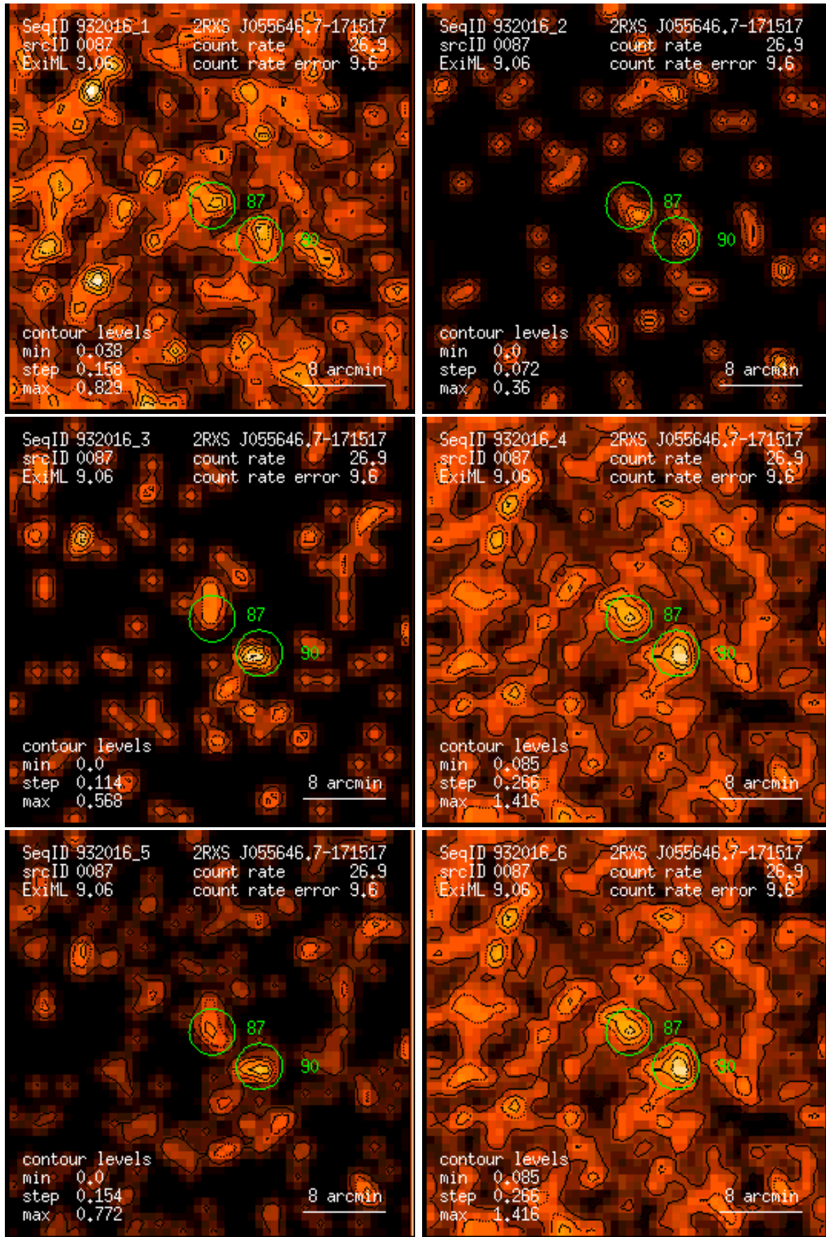
Figure 87: RASS 932016: detection 0087: band rate images, Gaussian filter: (1) PSPC channels 11 – 41, (2) 52 – 90, (3) 91 – 201, (4) 11 – 235, (5) 52 – 201, (6) 11 – 201. Broad band rates in counts/ks. Band rate contour levels in counts/ks/arcmin 2 .
